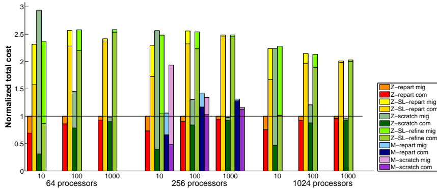
Fig. 7. Normalized total cost for cage15 with perturbed weights with \alpha = 10, 100, 1000 on 64, 256, and 1024 processors; colors indicate which repartitioning method was used.
