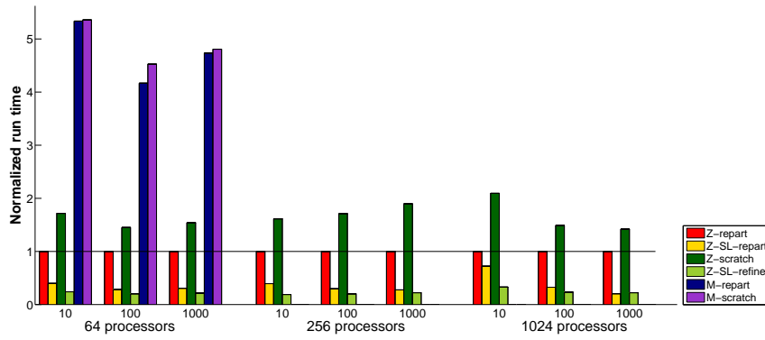
Fig. 8. Normalized run time with perturbed data structure for xyce680s with \alpha = 10, 100, 1000 on 64, 256, and 1024 processors; colors indicate which repartitioning method was used.
