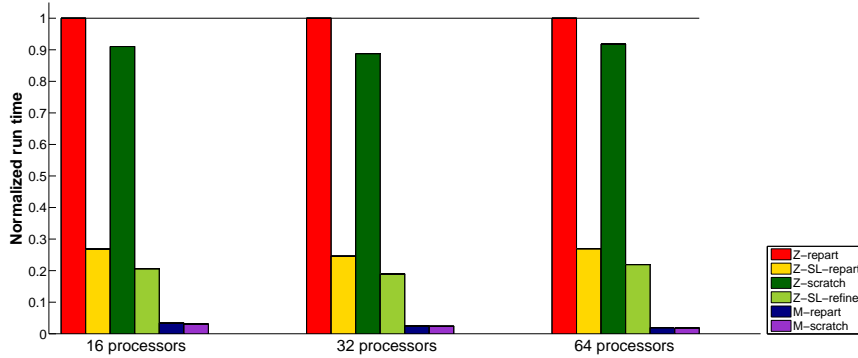
Fig. 16. Normalized run time for adaptive mesh refinement experiments with \alpha = 100 on 16, 32, and 64 processors; colors indicate which repartitioning method was used.
