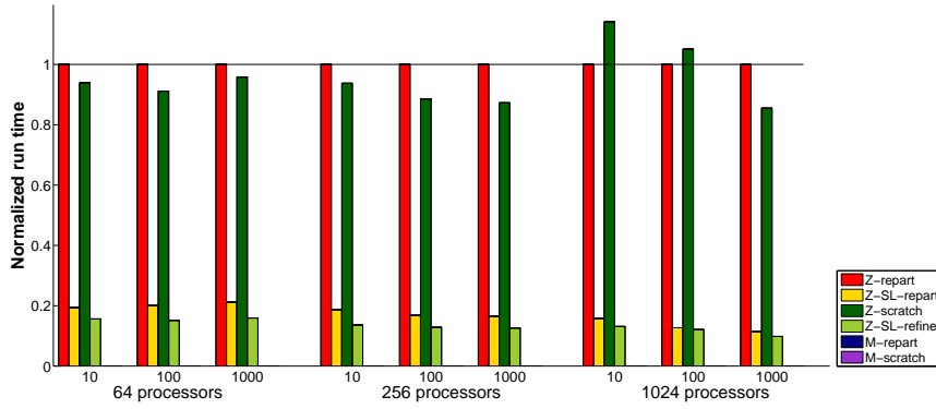
Fig. 12. Normalized run time with perturbed data structure for cage15 with \alpha = 10, 100, 1000 on 64, 256, and 1024 processors; colors indicate which repartitioning method was used.
