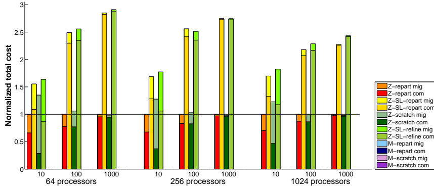
Fig. 6. Normalized total cost for cage15 with perturbed data structure with \alpha = 10, 100, 1000 on 64, 256, and 1024 processors; colors indicate which repartitioning method was used.
