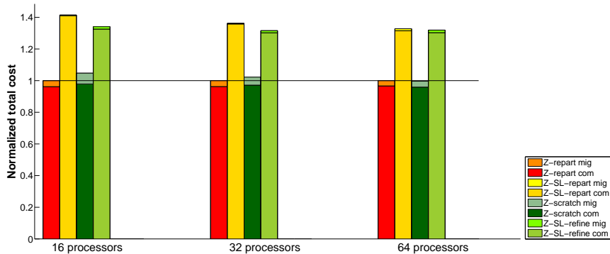
Fig. 17. Normalized total cost for term-by-document with \alpha = 100 on 16, 32 and 64 processors; colors indicate which repartitioning method was used.
