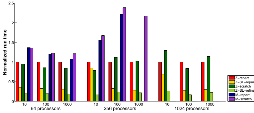
Fig. 9. Normalized run time with perturbed weights for xyce680s with \alpha = 10, 100, 1000 on 64, 256, and 1024 processors; colors indicate which repartitioning method was used.
