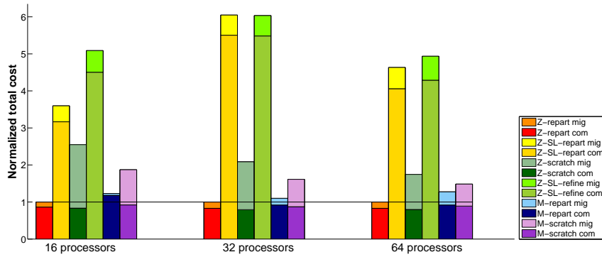
Fig. 15. Normalized total cost for adaptive mesh refinement experiments with \alpha = 100 on 16, 32 and 64 processors; colors indicate which repartitioning method was used.
