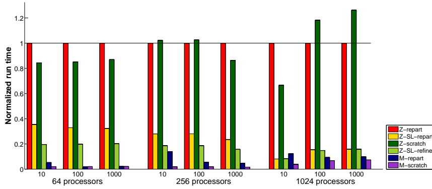
Fig. 11. Normalized run time with perturbed weights for slac6M with \alpha = 10, 100, 1000 on 64, 256, and 1024 processors; colors indicate which repartitioning method was used.
