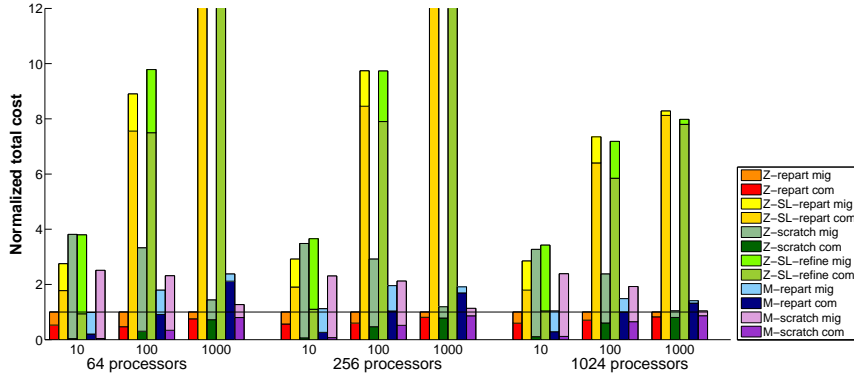
Fig. 5. Normalized total cost for slac6M with perturbed weights with \alpha = 10, 100, 1000 on 64, 256, and 1024 processors; colors indicate which repartitioning method was used. Z-SL-repart and Z-SL-refine bars are truncated to enhance readability.
