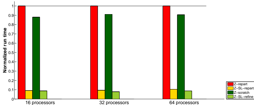
Fig. 18. Normalized run time for term-by-document with \alpha = 100 on 16, 32, and 64 processors; colors indicate which repartitioning method was used.
