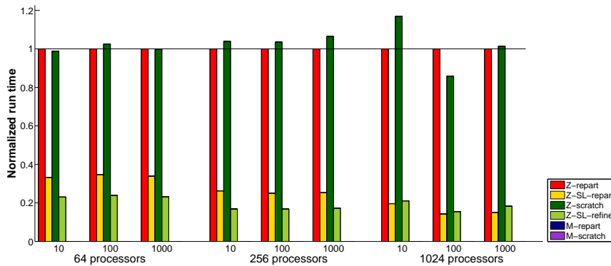
Fig. 10. Normalized run time with perturbed data structure for slac6M with \alpha = 10, 100, 1000 on 64, 256, and 1024 processors; colors indicate which repartitioning method was used.
