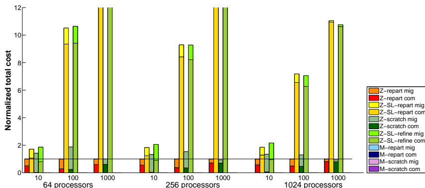
Fig. 4. Normalized total cost for slac6M with perturbed data structure with \alpha = 10, 100, 1000 on 64, 256, and 1024 processors; colors indicate which repartitioning method was used. Z-SL-repart and Z-SL-refine bars are truncated to enhance readability.
