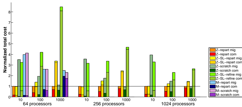
Fig. 2. Normalized total cost for xyce680s with perturbed data structure with \alpha = 10, 100, 1000 on 64, 256, and 1024 processors; colors indicate which repartitioning method was used.
