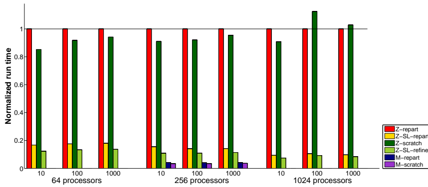
Fig. 13. Normalized run time with perturbed weights for cage15 with \alpha = 10, 100, 1000 on 64, 256, and 1024 processors; colors indicate which repartitioning method was used.
