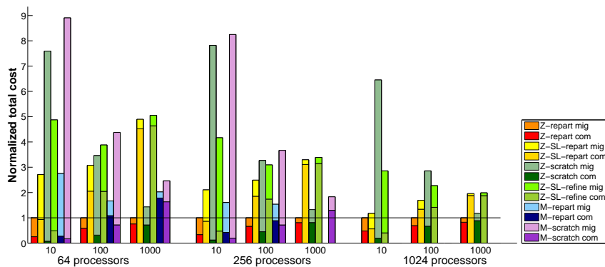
Fig. 3. Normalized total cost for xyce680s with perturbed weights with \alpha = 10, 100, 1000 on 64, 256, and 1024 processors; colors indicate which repartitioning method was used.
