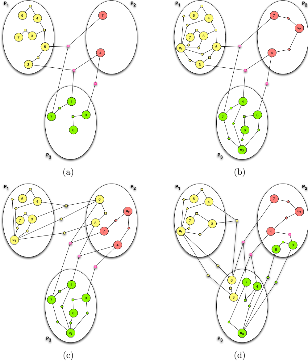
Fig. 1. (a): A sample computational hypergraph representation at the beginning of epoch j . Nets are depicted as squares and vertices are depicted as circles. The numbers inside the circles are the computational loads of each vertex. (b): Repartitioning hypergraph for epoch j ; for simplicity in the presentation, migration nets are depicted as diamonds and part vertices are depicted as octagons. (c) and (d): Two sample solutions with b_{comm} = 4, b_{mig} = 2 , and b_{comm} = 3, b_{mig} = 4 , respectively, under the assumption that the migration cost of each computation vertex and the application communication cost per net are one (i.e., each net's cost is one).
