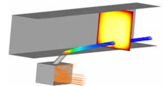
Simulation of a jet in crossflow
