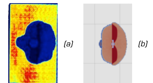
Figure 5. Composite panel tested under low velocity impact showing region of interlaminar delamination (a) ultrasonic scan and (b) modeled result
