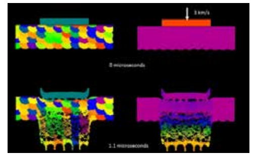
Figure 2. The simulated response of an additively manufactured specimen to a strong shock wave generated by the impact of a plate. The shock wave is created at the upper surface of the specimen where it is impacted. The wave moves downward and reflects off the lower surface. It interacts with the irregularities in the surface created by the manufacturing process. These irregularities form jets at the points of intersection between the “fish scales.” Extensive damage and fragmentation occurs in the interior of the specimen.
