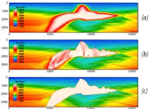
Given the seismic response from the synthetic SEG 2D Salt Model, ROL is used to recover the P-wave velocity field describing the subsurface. • (a) the initial guess of the velocity field • (b) the recovered velocity field, i.e., the subsurface model computed by ROL • (c) the "true" subsurface model. The (b) and (c) images are in good agreement except for below the salt, which has not been sufficiently "illuminated" with seismic waves.
