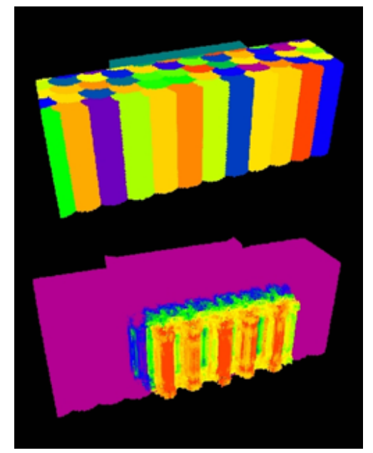
Figure 3. A cross-sectional view of the specimen from outside.
