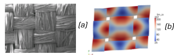
Figure 1. RVE of a fiber-reinforced composite sample (a) micrograph and (b) simulated
