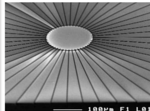
Perspective scanning electron microscope image of the front side of a 5 \mu\text{m} thick PV cell.
