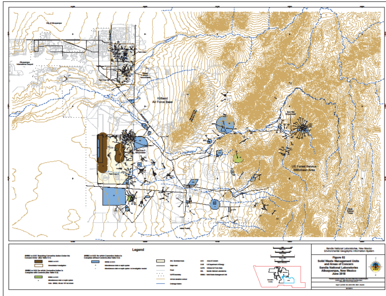
Figure 2 Location of Solid Waste Management Units and Areas of Concern, August 2018 Sandia National Laboratories, New Mexico
