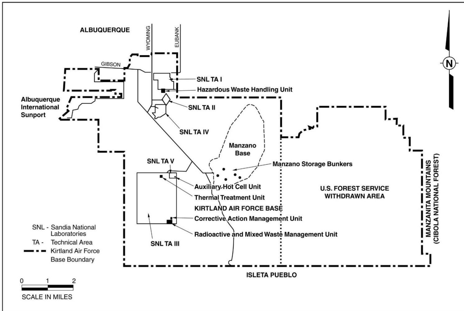
Figure 1 Location of Permitted Hazardous and Mixed Waste Units, August 2018 Sandia National Laboratories, New Mexico
