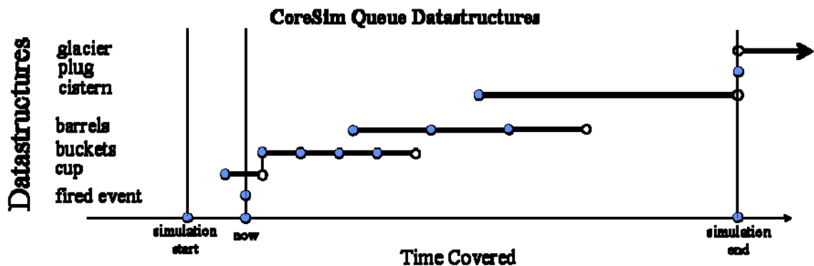
Caption: CoreSim's main discrete event loop employs a bucketing heuristic for queued events that dynamically exploits the frequency distribution of events. This
