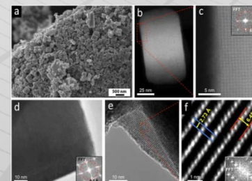
TEM and STEM Studies for Mo 6 S 8 Nanoparticles
