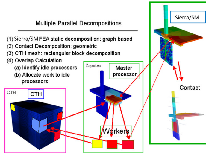
Fig. 8 Mesh decomposition and load balance for Zapotec coupling algorithm.
