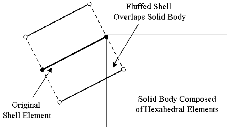
Fig. 7 Illustration of fluffed shell overlapping a solid structure.
