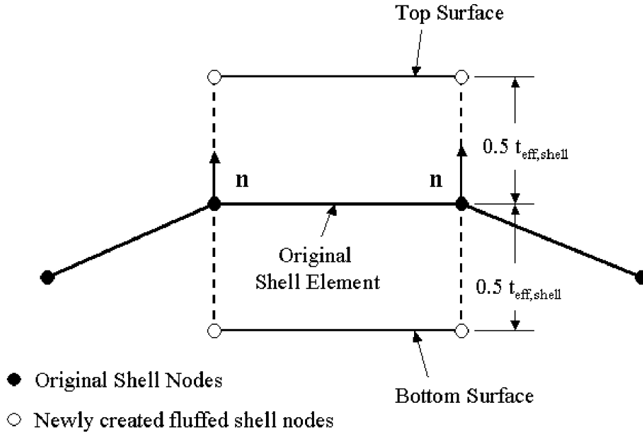
Fig. 5 Illustration of shell reconstruction algorithm.
