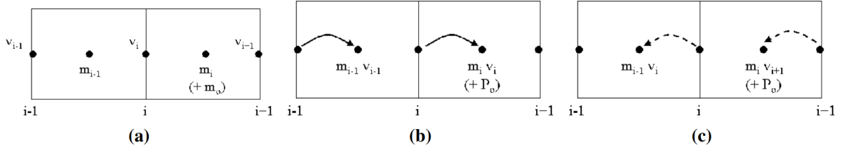
Fig. 3 Momentum insertion and recovery of face-centered velocities: (a) Primary mesh data before momentum shift, (b) Plus-shifted cell-centered momentum, P^+ , (c) Minus-shifted cell-centered momentum, P^- .
