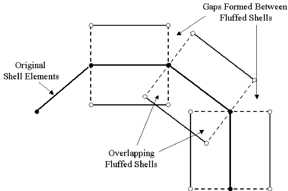
Fig. 6 Illustration of shell reconstruction algorithm for curved structures.
