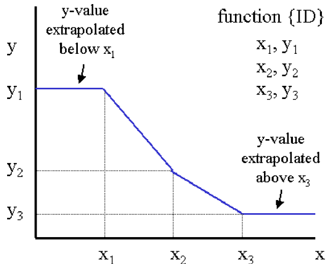
Fig. 9 Example of function definition.
