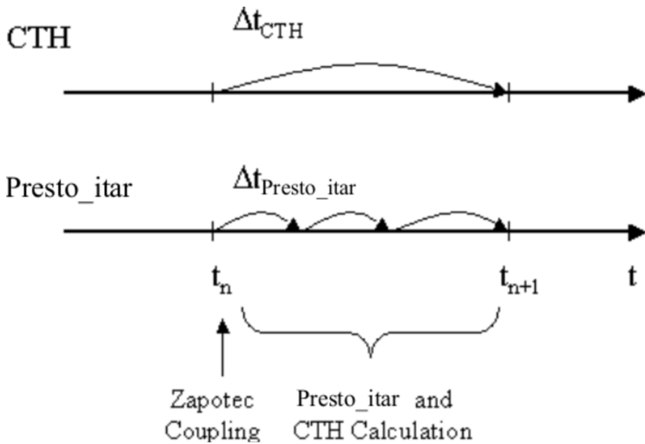
Fig. 2 Time synchronization of CTH and Presto_ITAR.
