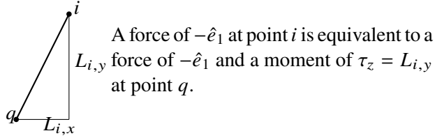
Figure 5-4. – Equilibration of loads.
