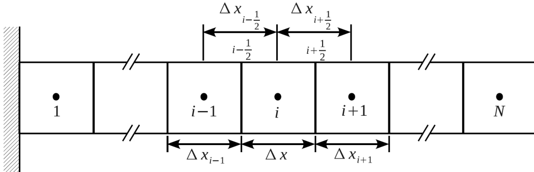
Fig. 3.7: Mesh index definition for 1-D composite fire boundary condition
