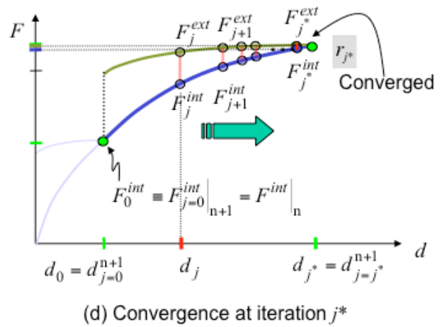
Fig. 13.1 Graphical depiction of nonlinear iterations.
