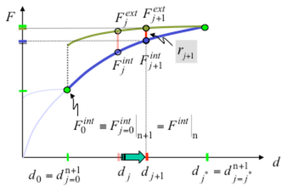
Fig. 13.1 Graphical depiction of nonlinear iterations.
