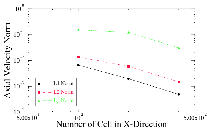
Figure 20.7-4.. Axial Velocity Norms for Coarse, Medium, and Fine Mesh Solutions
