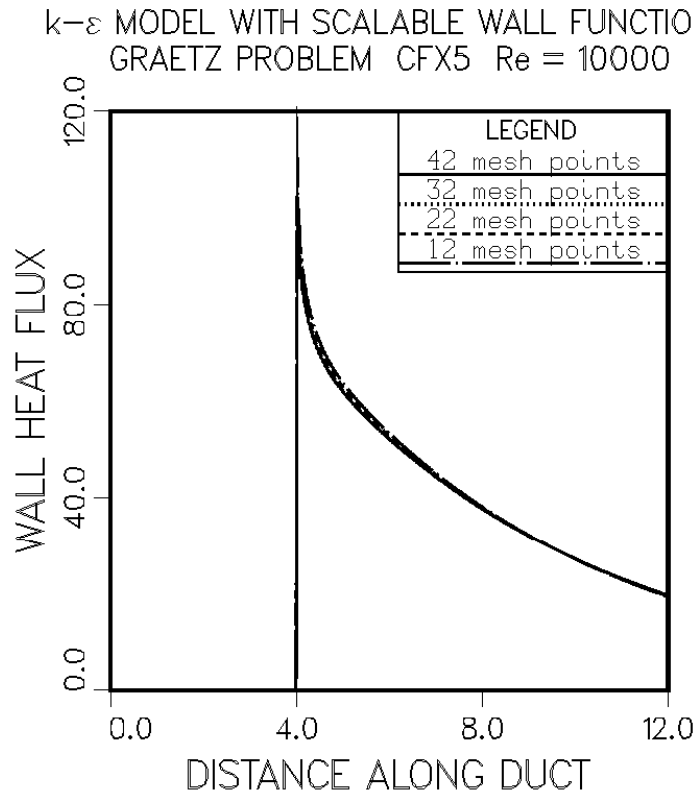
Figure 6.8-1.. Local heat flux distribution on heated channel wall: CFX results with different mesh spacing.
