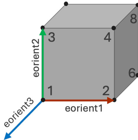
Figure 9-5. – Diagram of Eorient for a Hex8 element.
