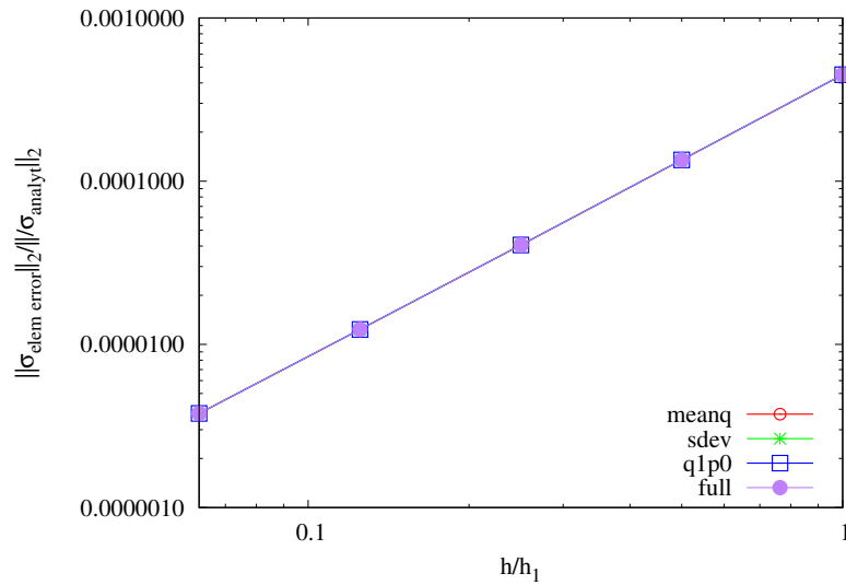
Figure 5-25. Stress convergence of the Newmark-beta method (trapezoidal rule—order 2), for each element formulation.
