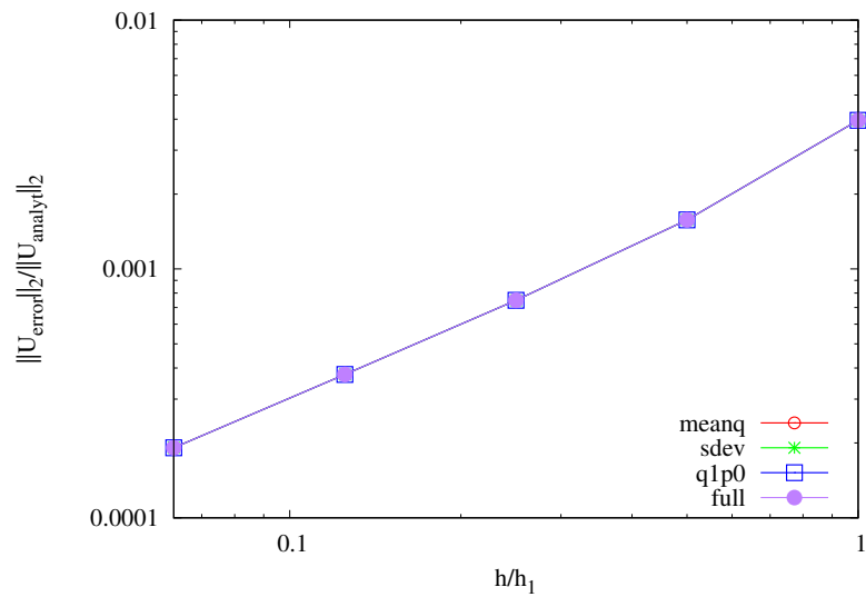
Figure 5-19. Displacement convergence of the HHT (order 2) method, for each element formulation.
