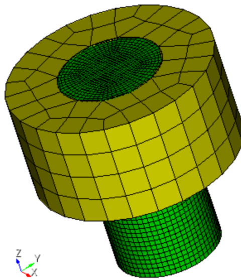
Figure 2-53. Geometry and mesh of the "mushroom" model.
