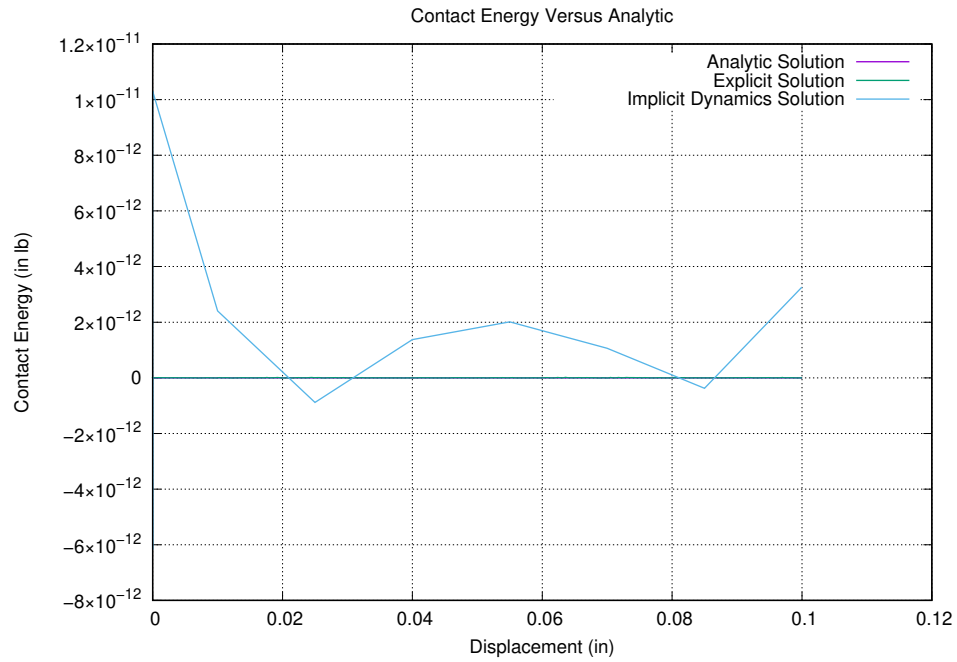
Figure 4-2. Energy-Displacement curve
