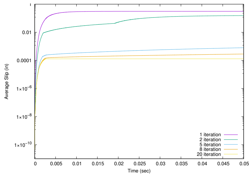
Figure 2-49. Average slip history of the middle wedge.
