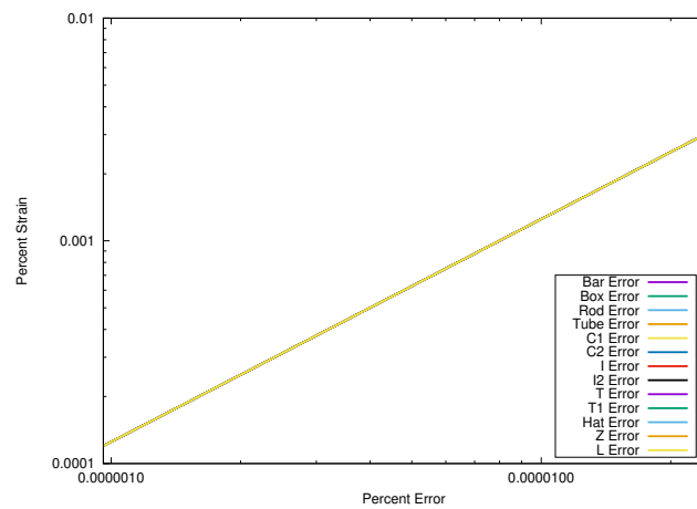
Figure 3-39. Log-Log plot of Strain vs Error
