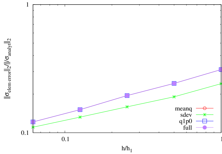
Figure 5-14. Stress convergence of the central difference method, for each element formulation.
