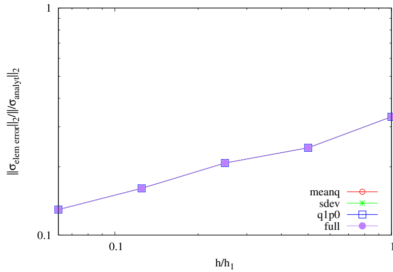
Figure 5-15. Stress convergence of the HHT (order 2) method, for each element formulation.
