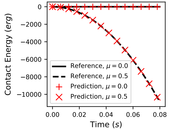
(b) Contact energy on a Hex8 inclined surface
