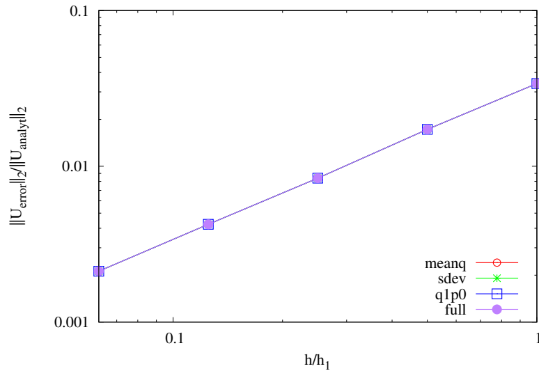
Figure 5-12. Displacement convergence of the HHT (order 2) method, for each element formulation.
