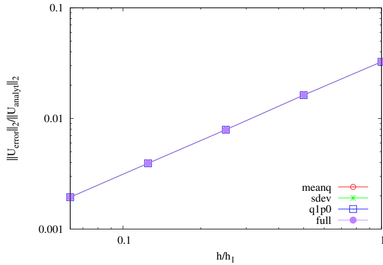
Figure 5-13. Displacement convergence of the HHT (order 1) method, for each element formulation.
