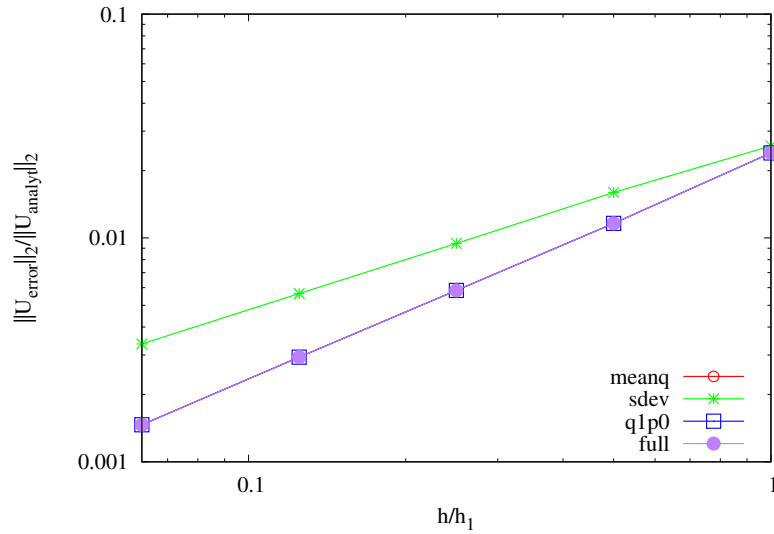
Figure 5-11. Displacement convergence of the central difference method, for each element formulation.
