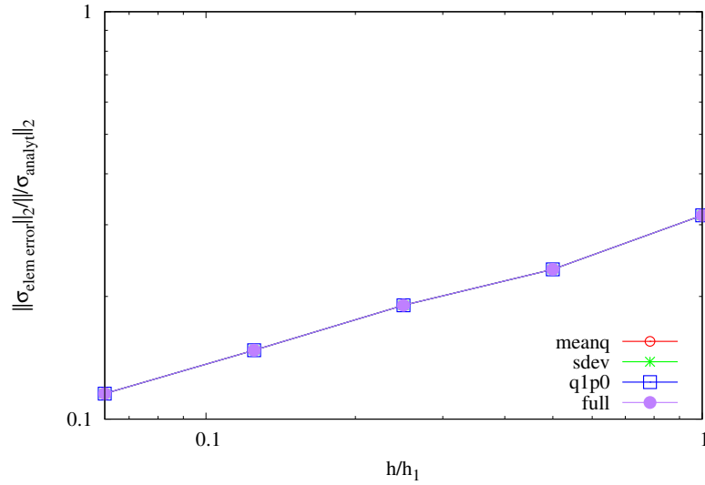
Figure 5-16. Stress convergence of the HHT (order 1) method, for each element formulation.
