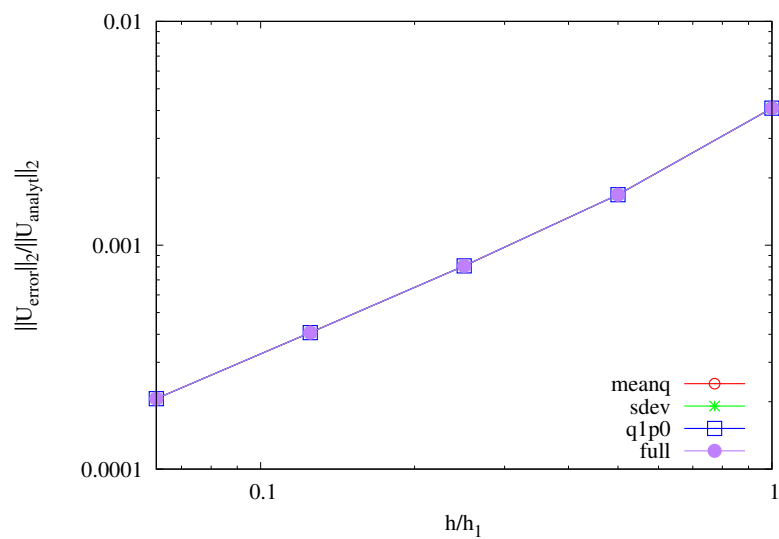
Figure 5-20. Displacement convergence of the HHT (order 1) method, for each element formulation.
