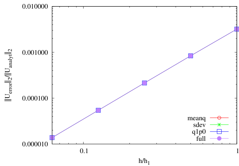
Figure 5-21. Displacement convergence of the Newmark-beta method (trapezoidal rule—order 2), for each element formulation.
