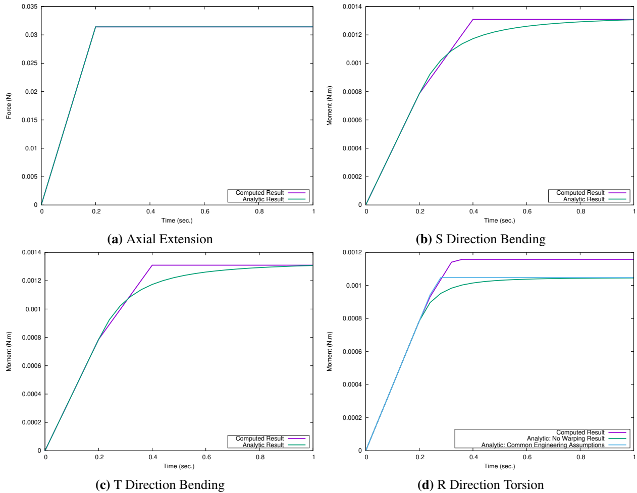
Figure 3-43. Rod Section
