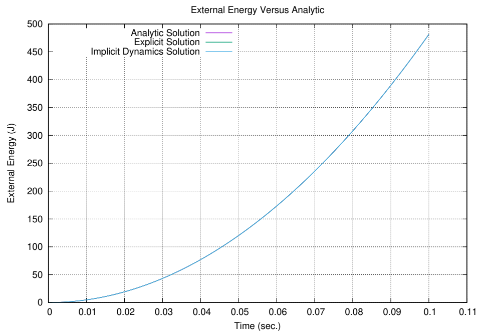
Figure 4-3. Energy-time curve
