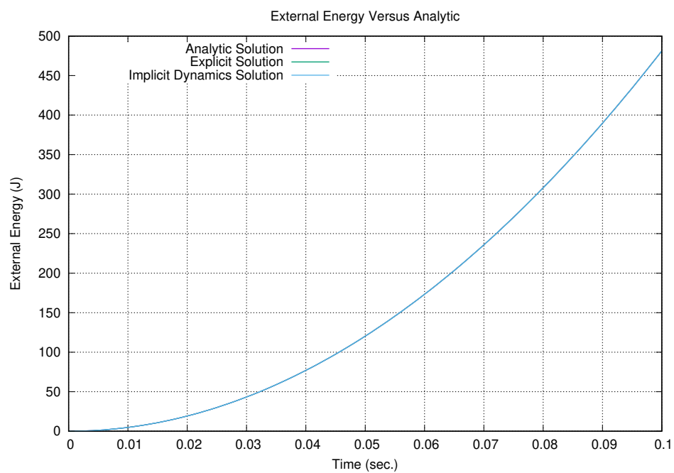
Figure 4-4. Energy-time curve
