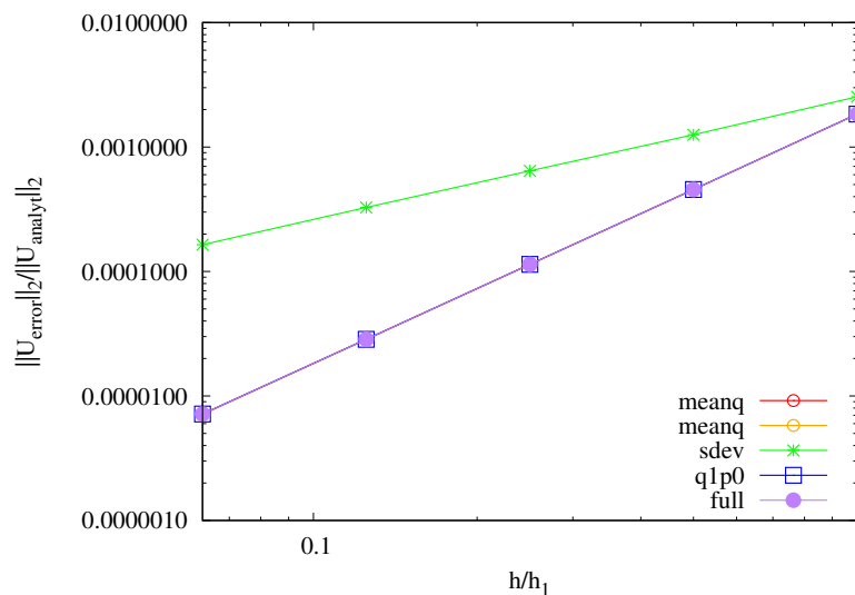
Figure 5-18. Displacement convergence of the central difference method, for each element formulation.
