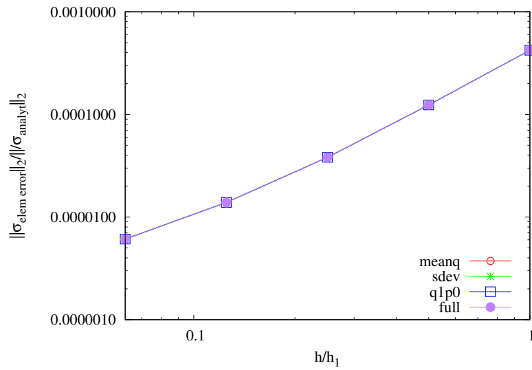
Figure 5-24. Stress convergence of the HHT (order 1) method, for each element formulation.
