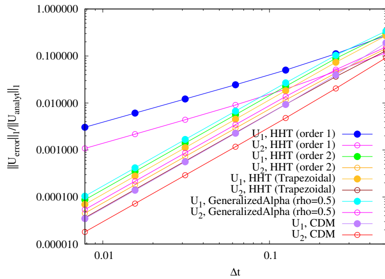
Figure 5-10. Convergence of the temporal integration cases, for each mass.
