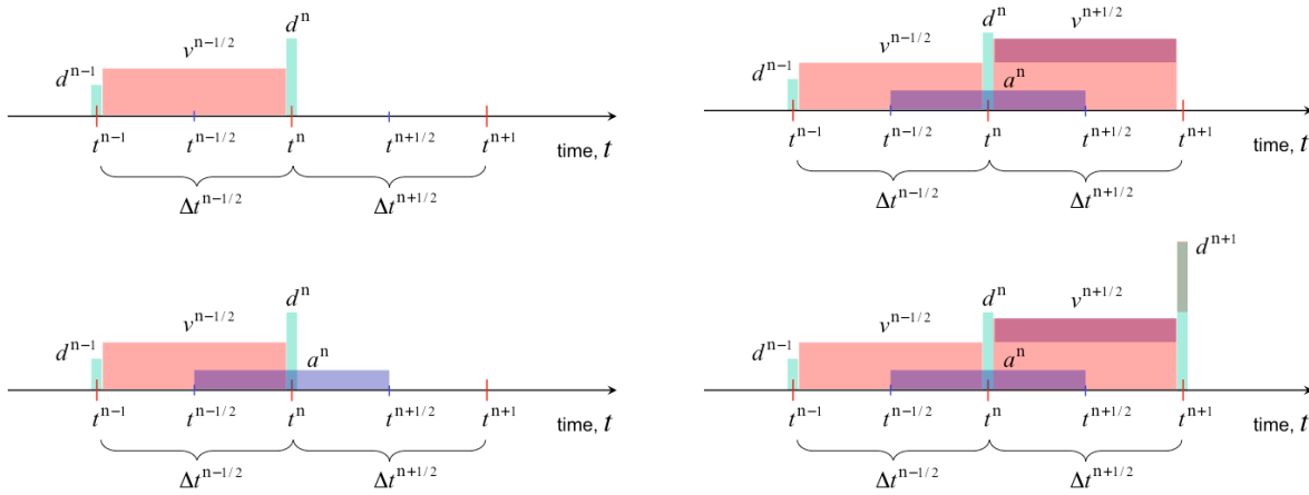
Fig. 12.3 Graphical representation of the central difference time integrator.
