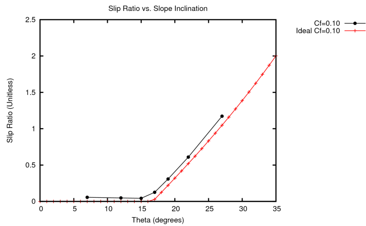
(b) Coefficient = 0.10
