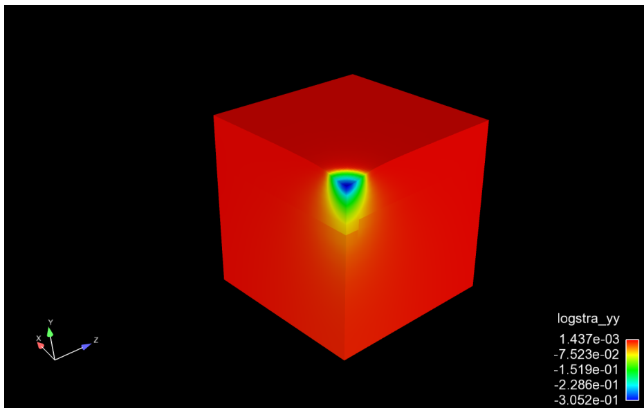
Figure 1-23. Final strain.
