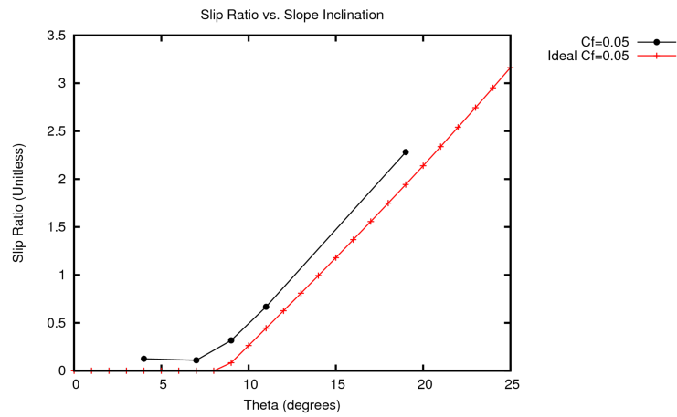
(a) Coefficient = 0.05
