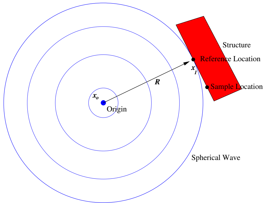
Figure 4-13. – Spherical Wave Geometry.
