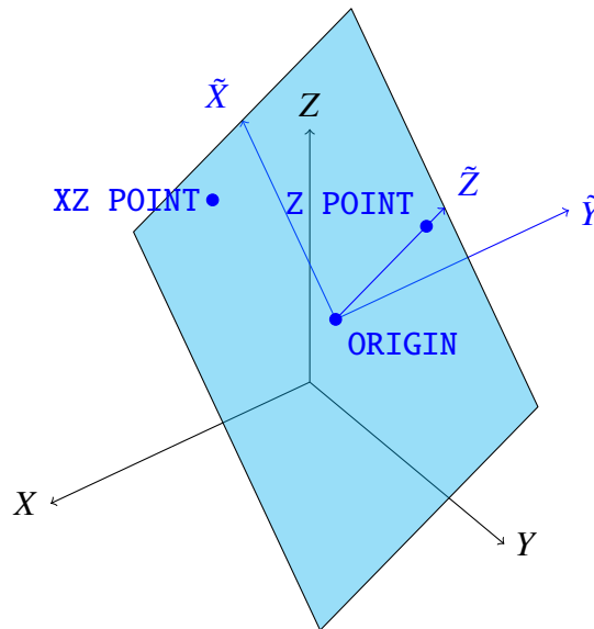
Figure 4-3. – Coordinate system definition vectors: note that XZ POINT determines the \tilde{X} axis, but need not lie along it, which is the case depicted in this figure.
