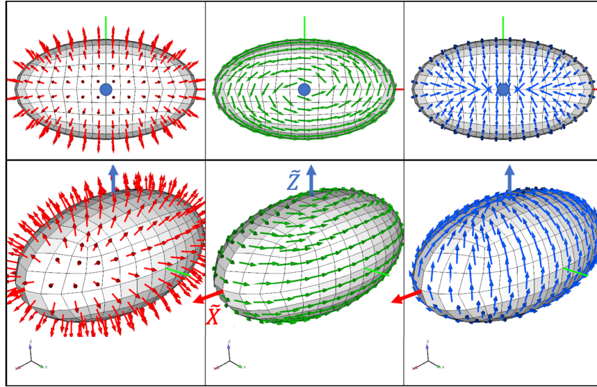
Figure 4-6. – Ellipsoidal Coordinate System Using \text{axis\_stretching} = (2.0, 1.1, 1.0) . \hat{r} is red, \hat{s} is green, and \hat{t} is blue.
