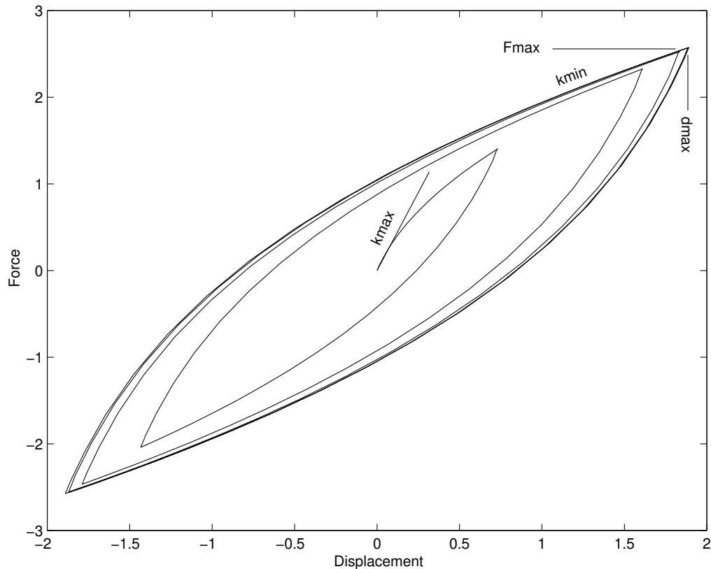
Figure 7-13. – Hys element parameters.
