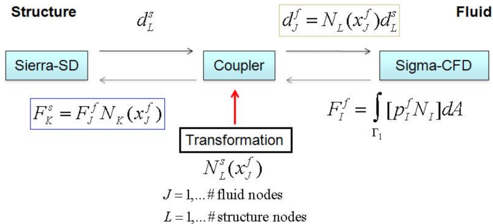
Figure 4-14. – Fluid-Structure Interaction (FSI) Infrastructure.
