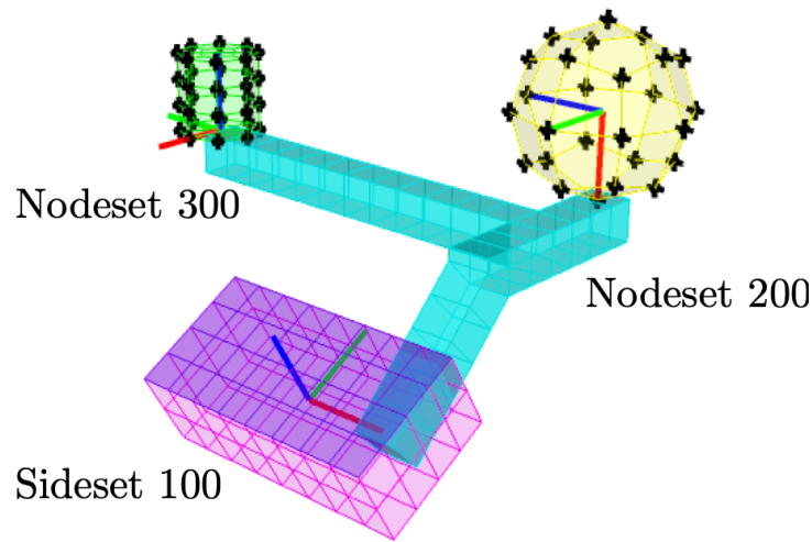
Figure 4-8. – An example of how coordinate systems are used. Accelerations are measured on the sphere (nodeset 200) due to a radial force applied on the cylinder (nodeset 300).
