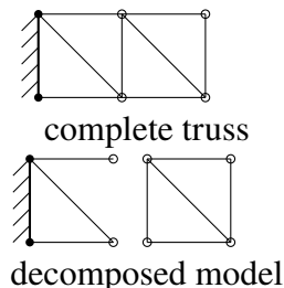
Figure 3-2. – Truss Decomposition Issues.
