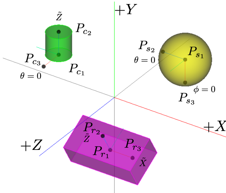
Figure 4-4. – Three examples (rectangular, spherical, and cylindrical) of transformed coordinate systems are given. The center of the rectangular block ( 6 \times 2 \times 3 ) is located at (3, -1, 5) , and rotated 30 degrees about the X axis. The center of the sphere (radius of 2) is located at (5, 4, -2) . The center of the cylinder (radius of 1, height of 2, and rotated 90 degrees about the X axis) is located at (-5, 2, 0) . The new coordinate systems are defined respectively of each of the geometries, and are indicated by \tilde{X} \tilde{Y} \tilde{Z} and the subscripts ( r , s , and c ).
