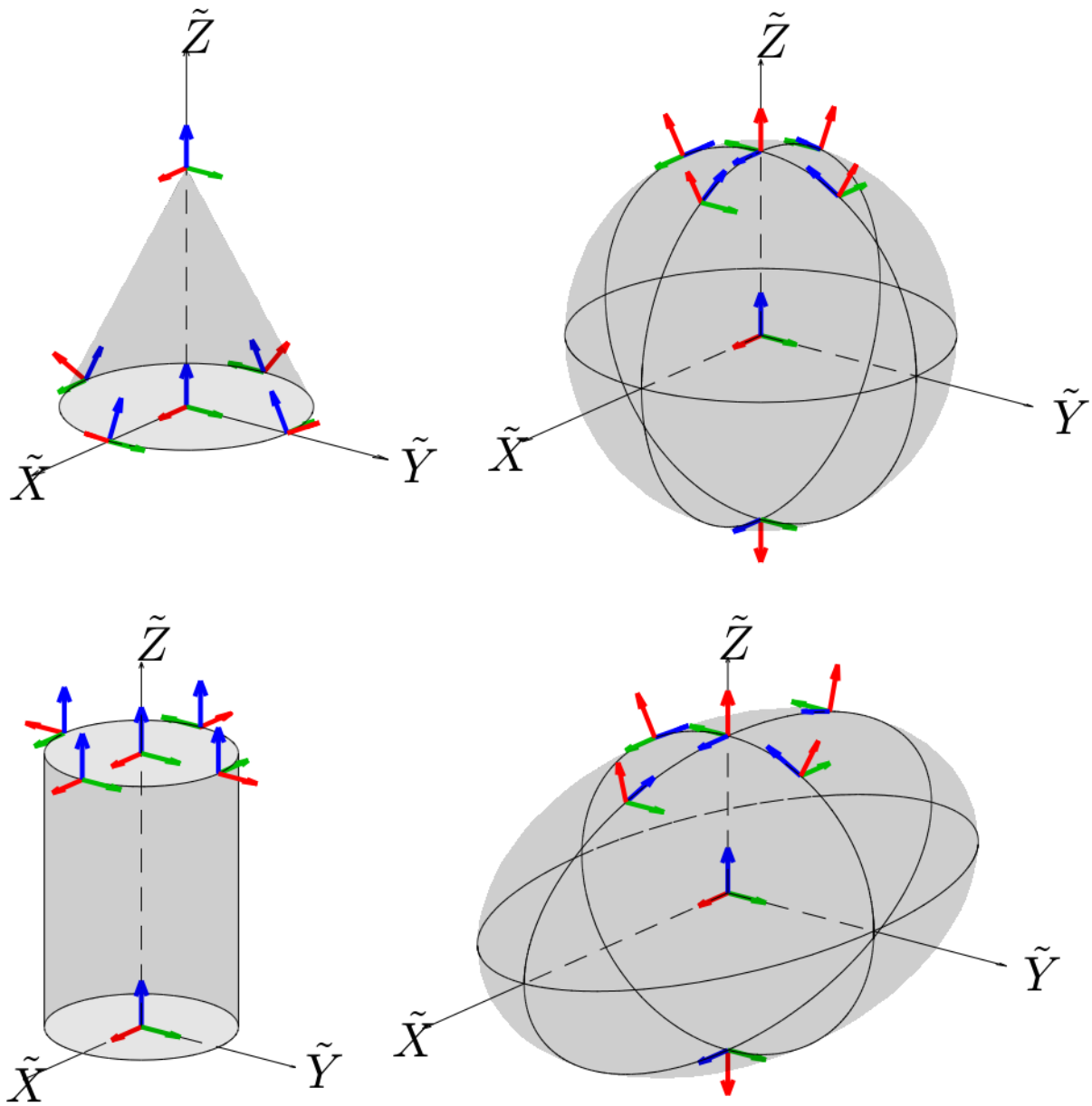
Figure 4-7. – Coordinate system behavior near the \tilde{Z} axis. \hat{r} is red, \hat{s} is green, and \hat{t} is blue.
