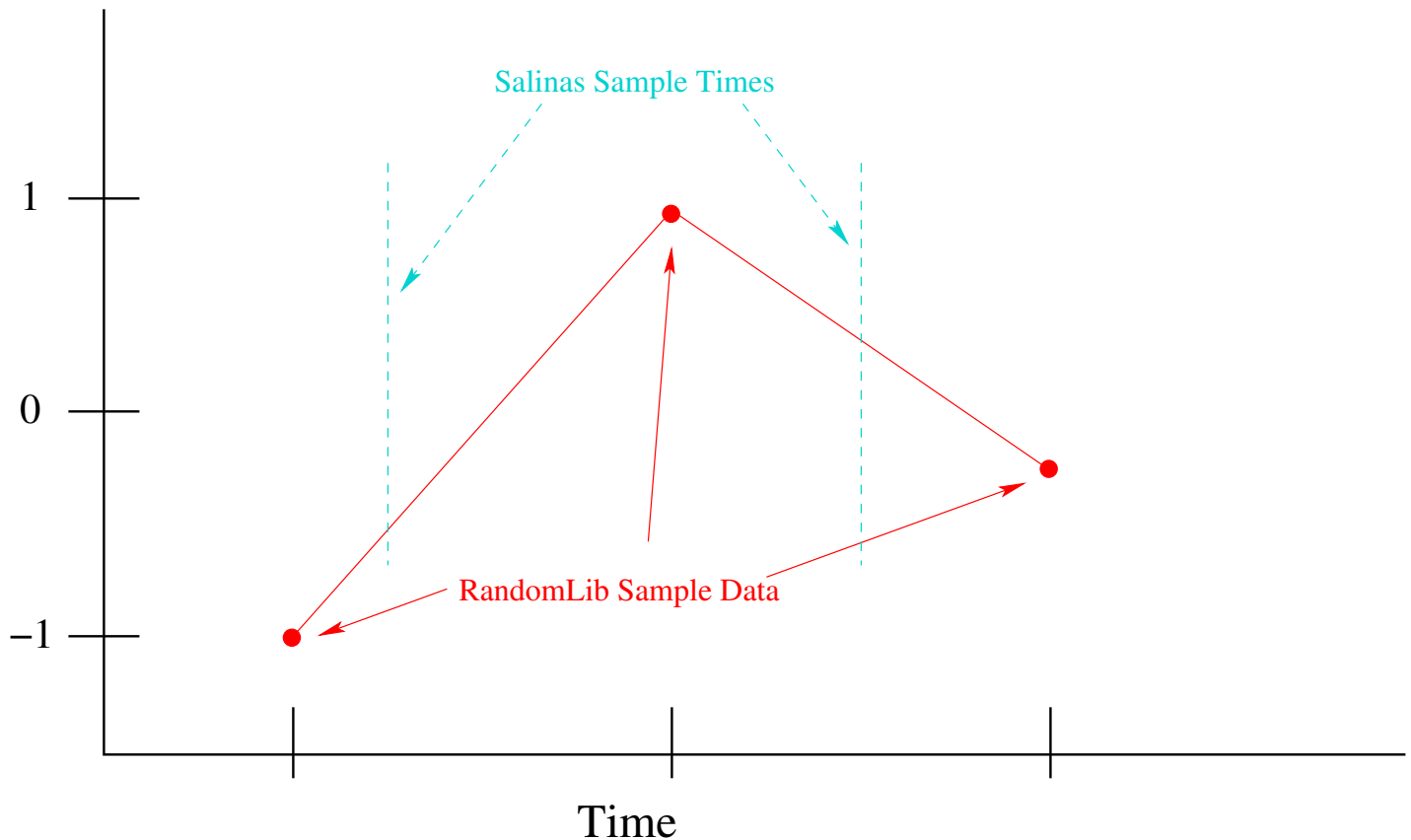
Figure 4-12. – RandomLib Temporal Interpolation. Because of different time steps in the RandomLib data library and the Sierra/SD time step algorithm, the function value returned depends on the time interpolation algorithm. With interp=none , the first value returned to Sierra/SD is about -1.0, as that is the nearest time sample in the data. With interp=linear , the value returned is about -0.6. Note that round off can cause odd behavior with interp=none , even if the two data sets have the same fundamental time step.
