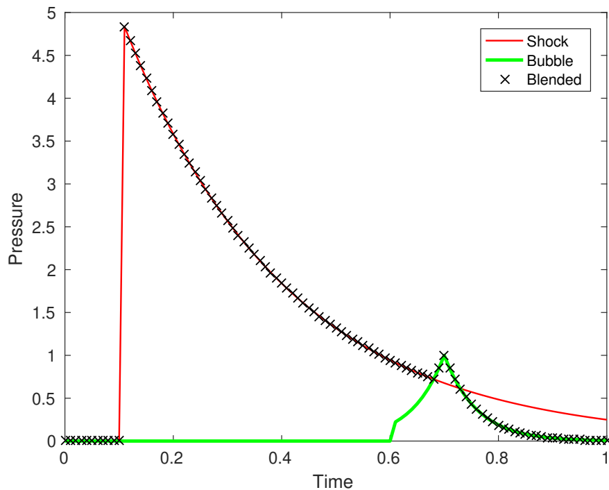
Figure 4-15. – Illustration of first crossing blended function.
