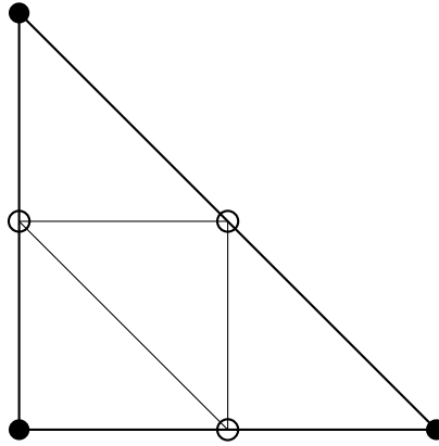
Figure 7-3. – Tria6 Element.
