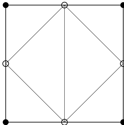
Figure 7-2. – Quad8T Element.
