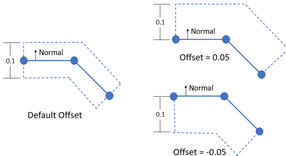
Figure 7-9. – Offset examples for shell of thickness 0.1.
