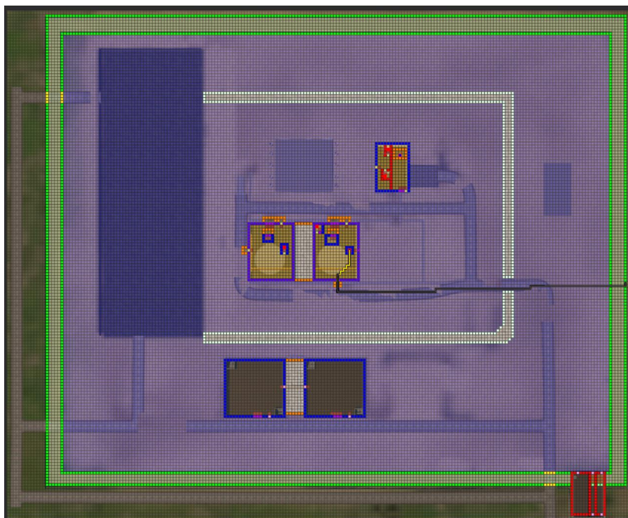
Figure 19. Above-Grade Reactor Sabotage Attack Pathway
