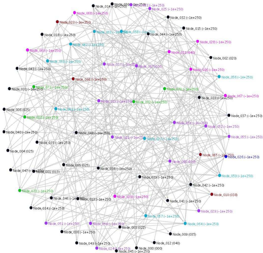
Figure 25. The expected social network \langle \mathcal{G} \rangle , drawn from data collected during the first 40 days, for Problem II. Nodes represent the 74 members of the population and are colored by their compound affiliations. Links in the graphs represent the cross-compound social links seen in 50% (or higher) of the samples.
