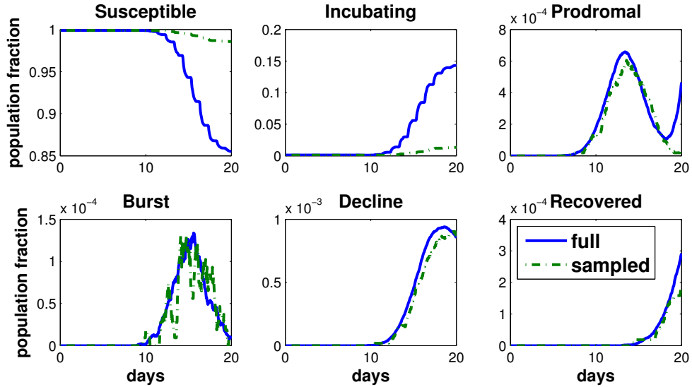
Figure 5. Smallpox epidemic: population fraction in each disease stage, comparing full-fidelity dynamic network to reduced-order network obtained via person-to-location clustering, Data Set Version 1.0.
