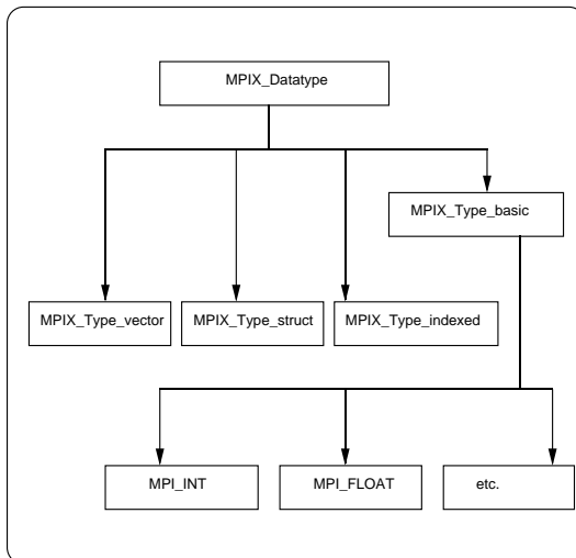
Figure 12: Hierarchy of Datatype-Based Classes in MPI++
