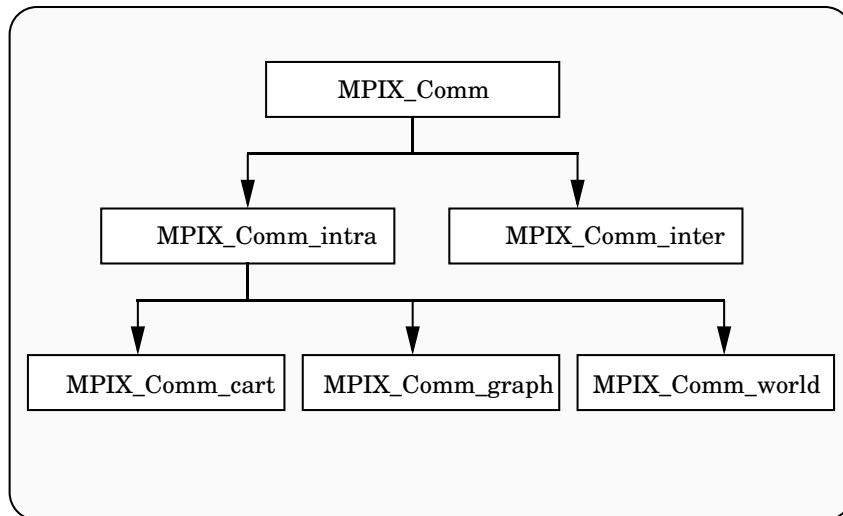
Figure 7: Hierarchy of Communicator-Based Classes for MPI++
