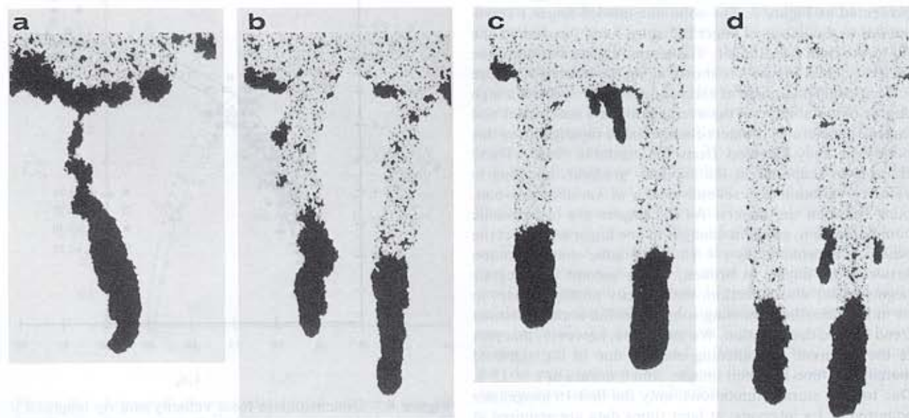
Figure 6. Effects of gravitational gradient on finger development. Images were selected such that L_i was of a similar magnitude. (a) Experiment 6, G_g = 0.25 , L_i = 9.08 cm, and t = 1518 s. (b) Experiment 2, G_g = 0.50 , L_i = 9.85 cm, and t = 104 s. (c) Experiment 8, G_g = 0.75 , L_i = 9.43 cm, and t = 31 s. (d) Experiment 13, G_g = 1.00 , L_i = 8.99 cm, and t = 23 s.
