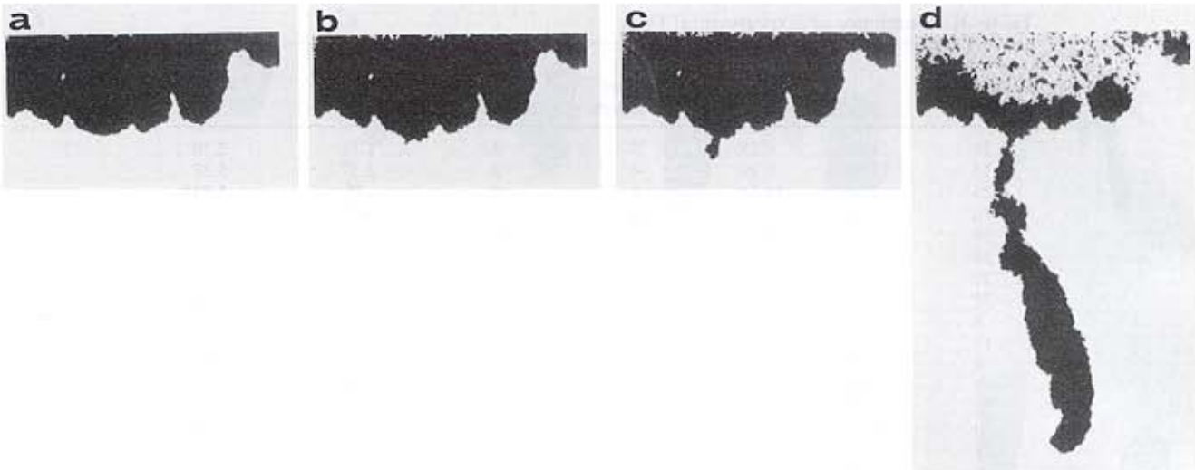
Figure 4. Percolation-type development of an unstable front, experiment 6 ( G_g = 0.25 , L_i = 9.08 cm). (a) Front is shown near the end of stable imbibition ( t = 39 s). (b) Several minutes after the cessation of imbibition the front is nearly frozen in place, limited movement is occurring as local apertures are successively drained and spanned in a sequence of individual Haines jumps; note the small tendril forming on the largest perturbation ( t = 619 s). (c) Movement continues on a discrete basis; however, the rate of drainage/filling is visibly increasing ( t = 1069 s). (d) After L_f reaches a critical threshold, flow ceases to be on a discrete basis as observed at earlier times, leading to rapid formation of the finger shown ( t = 1518 s).
