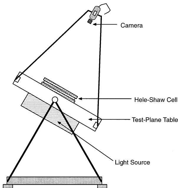
Figure 3. Experimental apparatus showing Hele-Shaw cell on the rotating test stand.
