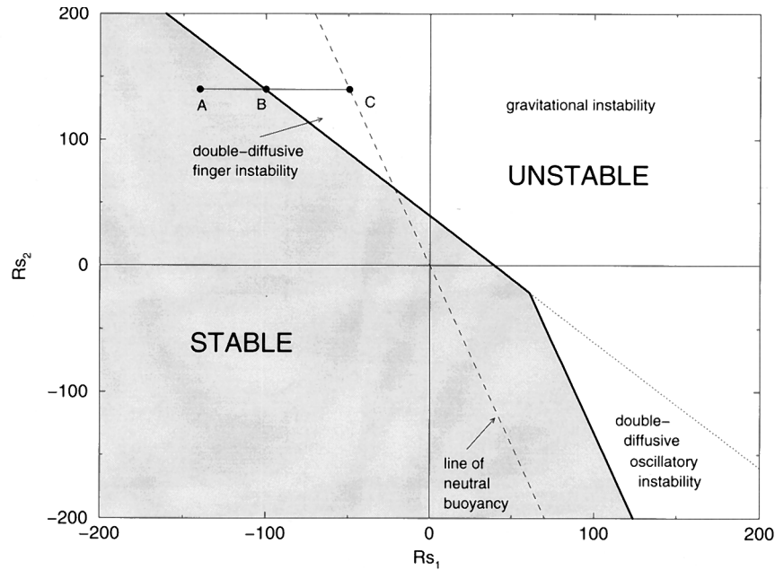
Figure 1. Stability plot in solutal Rayleigh number space that shows the location of the possible types of transport phenomena, as determined by Nield [1968] and Nield and Bejan [1992], for double-diffusive transport in a horizontally infinite porous medium bounded by two impermeable boundaries of constant solute concentration. The shaded and unshaded areas denote regions of hydrodynamic stability and instability, respectively. For a given porous medium and \beta_2 \Delta c_2 , point A on the dotted line exists in a stable region, and transport occurs by diffusion alone. An increase in \beta_1 \Delta c_1 leads to double-diffusive finger convection initiating at point B. Further increase within the double-diffusive convection regime past C causes the fluid to reach neutral buoyancy, resulting in motion that is probably driven by both density and double-diffusive instabilities, until at \beta_1 \Delta c_1 = 0 , only one solute is present, and Horton and Rogers' [1945] and Lapwood's [1948] criterion for density-driven convection is reached ( Rs_2 \geq 4\pi^2 ). As \beta_1 \Delta c_1 is increased from zero, both solutes are destabilizing, no double-diffusive motions can occur, and transport is driven by the positive upward density gradient of both solutions. Oscillatory convection occurs in the fourth quadrant ( Rs_1 positive and Rs_2 negative); at large absolute values of Rs_1 and Rs_2 , the transition from oscillatory to a direct instability mode is, however, no longer defined by (2) [ Baines and Gill , 1969].
