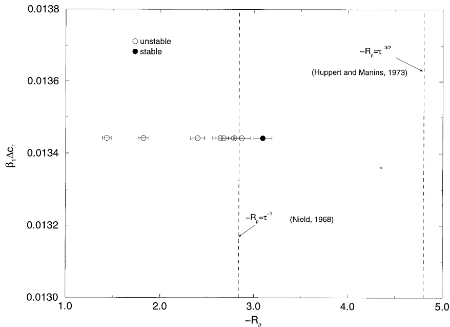
Figure 7. Initial conditions and result of each experiment in the space of \beta_1\Delta c_1 and -R_\rho . Open circles represent unstable experiments that resulted in fingering, while the closed circle represents the stable experiment. Nield's [1968] simplified analysis suggests instability for -R_\rho < 2.84 , while Huppert and Manins' [1973] analysis suggests instability for -R_\rho < 4.8 .
