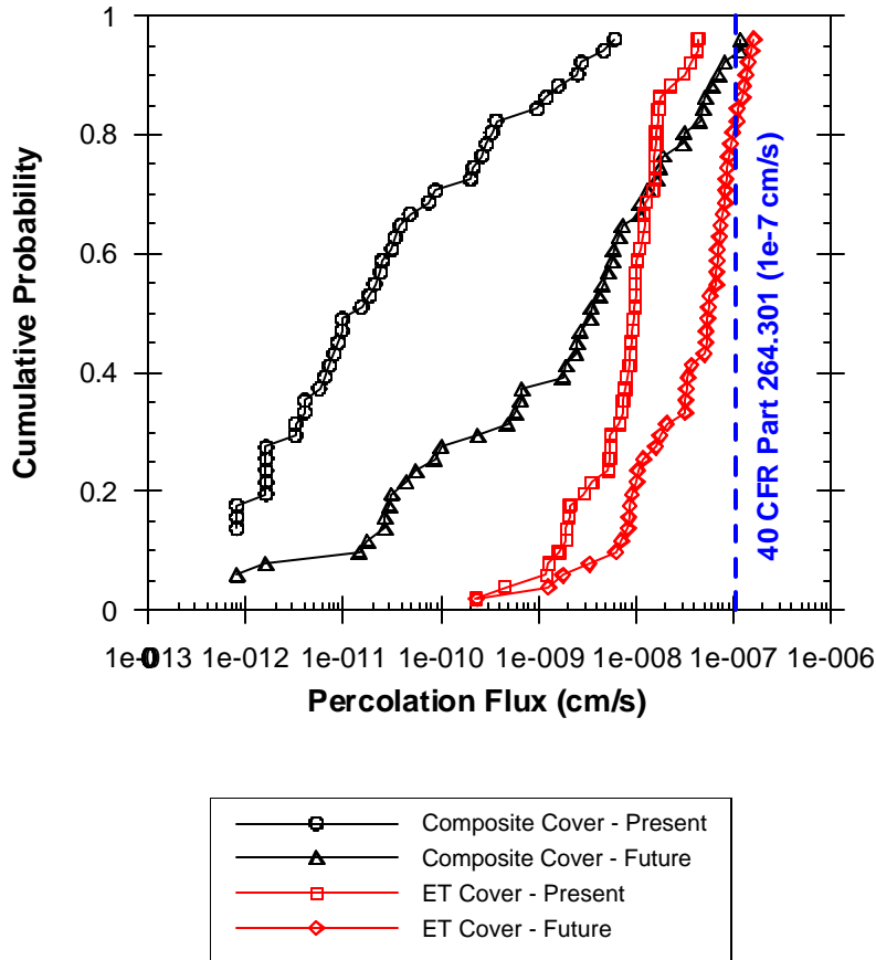
Figure 14. Cumulative probability distribution of water percolation reaching the mill tailings for present and future conditions (scenarios 1 and 2) and for the evapotranspiration cover.
