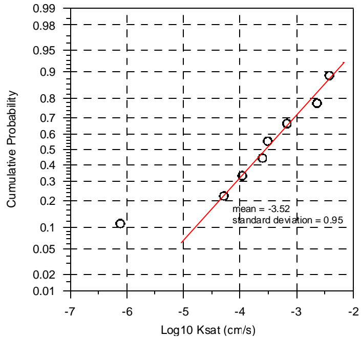
Figure B-1. Cumulative probability of log-transformed hydraulic conductivity for soil samples of layer 1.
