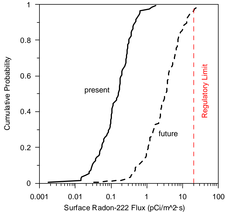
Figure 10. Cumulative probability distribution of simulated radon flux at the land surface for present and future conditions (scenarios 3 and 4).
