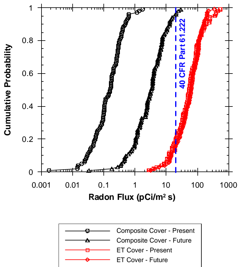
Figure 15. Cumulative probability distribution of radon-222 flux at the landfill cover for present and future conditions (scenarios 3 and 4) and for the evapotranspiration cover.
