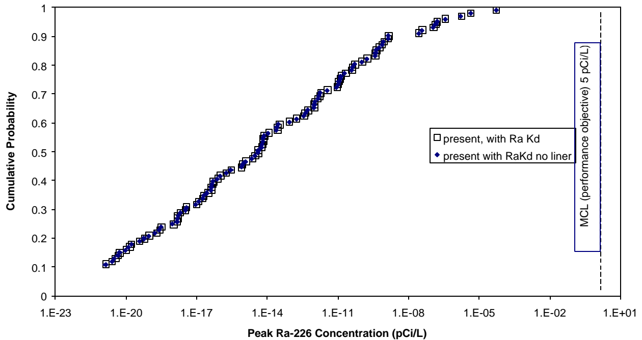
Figure 19. Peak Ra-226 concentration in the shallow aquifer during present-day conditions using the evapotranspiration cover with and without a double composite-liner system beneath the mill tailings.
