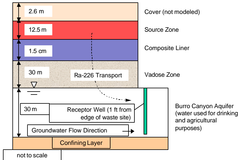
Figure 7. Conceptual model for radionuclide transport from the mill tailings to the deep Burro Canyon aquifer and location of receptor well for present (scenario 7) and future (scenario 8) conditions.
