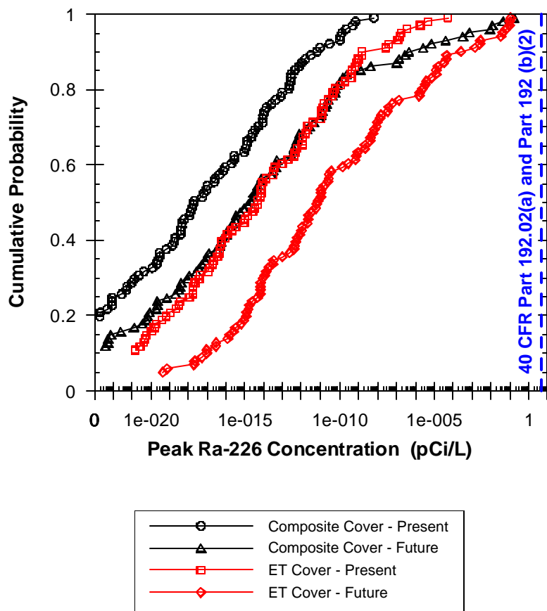
Figure 16. Cumulative probability distribution of Ra-226 concentration in the shallow alluvial aquifer for present and future conditions (scenarios 5 and 6) and for the evapotranspiration cover.
