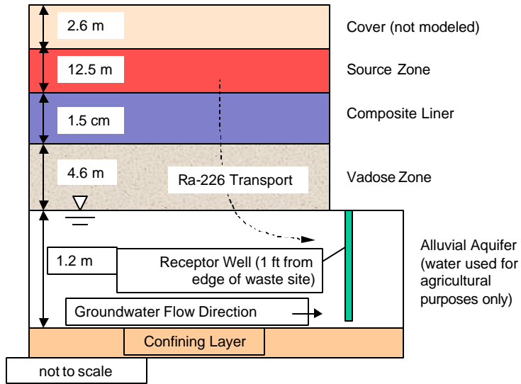
Figure 6. Conceptual model for radionuclide transport from the mill tailings to the shallow alluvial aquifer and location of receptor well for present (scenario 5) and future (scenario 6) conditions.
