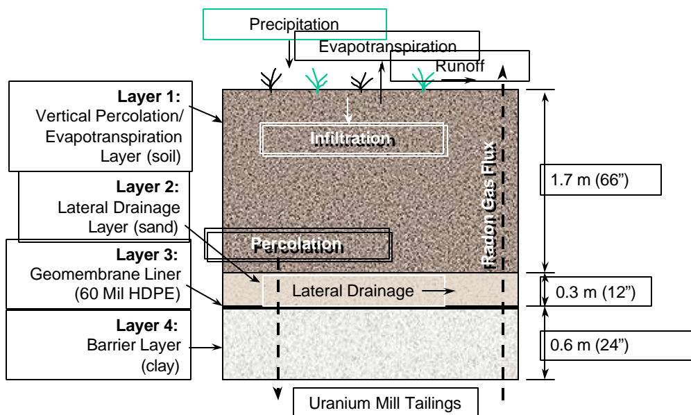
Figure 5. Conceptual model for water percolation (scenarios 1 and 2) and gas transport (scenarios 3 and 4) through a composite (base-case) cover design for present and future conditions. A 3% slope is assumed for the drainage layer. An alternative evapotranspiration (ET) cover design that only consists of Layer 1 is also considered in Section 4.5.
