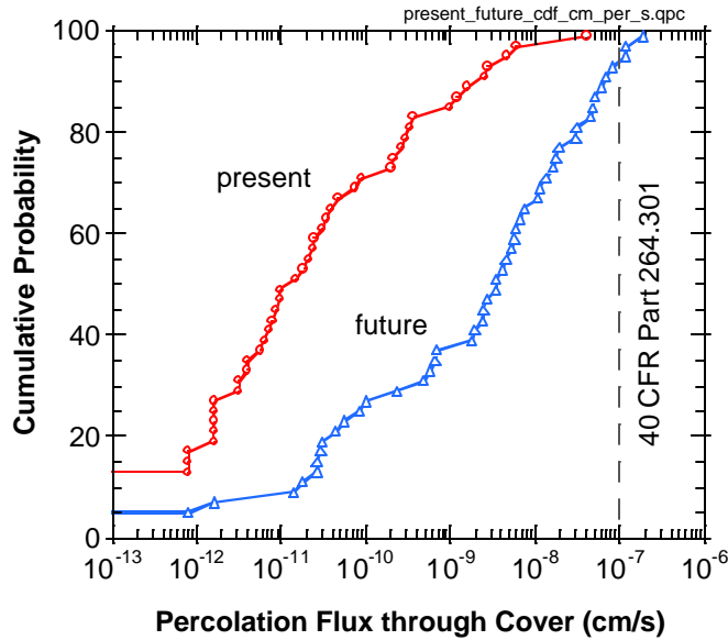
Figure 9. Cumulative probability distribution of water percolation reaching the mill tailings for present and future conditions (scenarios 1 and 2).
