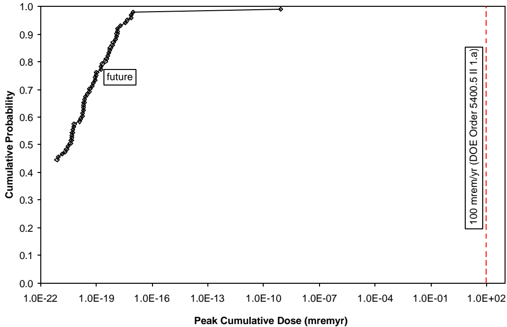
Figure 13. Cumulative probability distribution for peak cumulative dose for Ra-226 and its progeny from the Burro Canyon aquifer for future conditions (scenario 8). Note: dose values of 0 are not plotted on the log scale.
