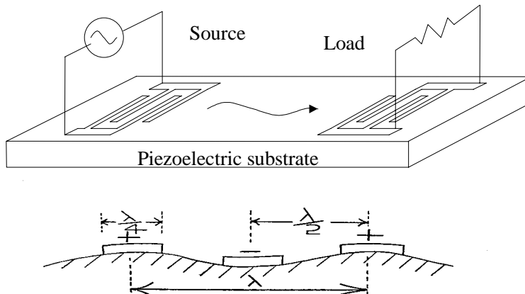
Figure 1: Surface Acoustic Wave Device
