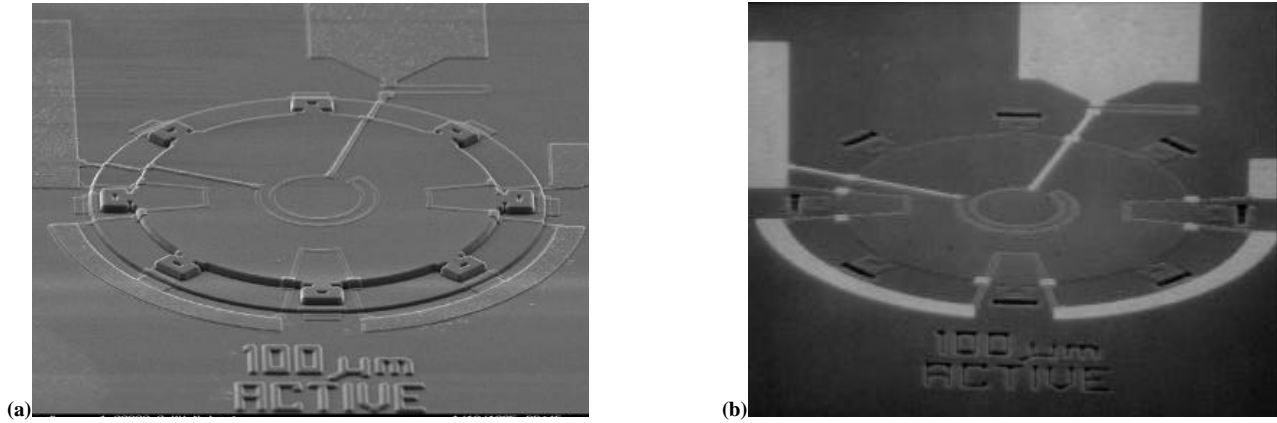
Figure 3. (a) Non-planar and (b) planar pressure sensor diaphragms. Etch access ports on planar sensor are approx. 0.8 μm deep, but do not cause processing difficulties with photolithography, dry etch, or metallization. Diaphragms are 100 μm in diameter.
