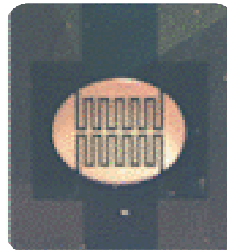
Figure 2. Microhotplate.
