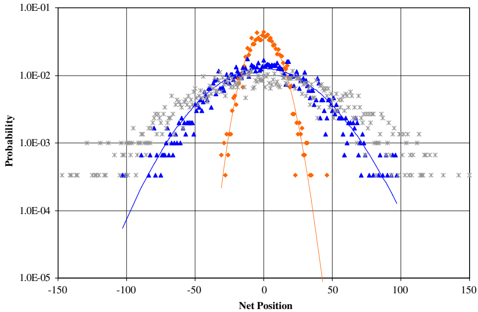
Fig. A.1. Observed frequency distributions of 1000 observations of net position at time 1000 for the random walk (grey symbols), and the finite deposit model with D_i(0) = 1000 (blue symbols) and D_i(0) = 100 (orange symbols). Analytical curves for the steady-state distribution (Eq. (A.1)) are included for the finite deposit model.
