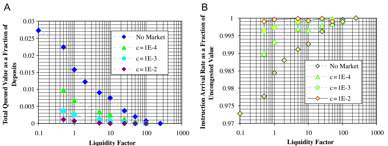
Fig. 12. Fraction of deposits in payment queues vs. liquidity factor (A) and instruction arrival rate as a fraction of the rate in an uncongested system (B) for three values of market conductance. Results for the no-market case are included for comparison. Lines are included as a visual aid. In each case the fractional reduction in instruction arrival is, allowing for sampling error, equal to the fraction of deposits held in queues.
