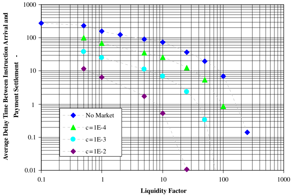
Fig. 13. Average delay time between instruction arrival and settlement vs. liquidity factor for three values of market conductance. Increasing market conductance lowers delay time with the most marked reduction seen for c larger than 10^{-4} .
