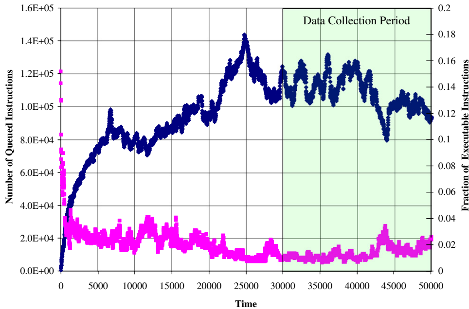
Fig. 2. Average total number of queued instructions (blue symbols, left axis) and fraction of instructions that can be immediately executed (pink symbols, right axis) in successive time intervals of size 10 for a liquidity factor of 1 using the primitive model. Data for the primitive system were collected after a time of 30 000 to minimize the influence of start-up transients.
