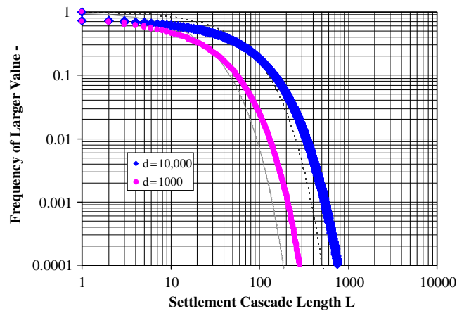
Fig. 20. Frequency distribution of observed settlement cascades for a liquidity factor of 1 and two values of deposit level. Analytical approximations for each distribution based on Eq. (18) are shown in light grey lines.
