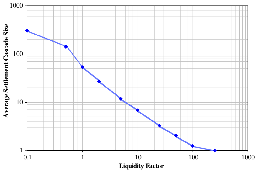
Fig. 5. Average length of settlement cascades observed in a time interval of size 20 000 for several values of the liquidity factor. Line indicates the analytical approximation for the expected value of cascade size from Eq. (16). The analytical approximation was only evaluated at the liquidity factor values used in the simulations: the line is a visual aid.
