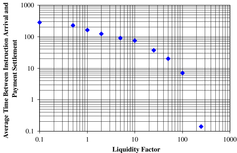
Fig. 8. Average delay time between instruction arrival and settlement vs. liquidity factor. The average delay time is calculated as the ratio of the number of queued payments to the rate of instruction arrival. A delay time of 1 means that the average time between an instruction's arrival and the ensuing payment is the same as the average time between instruction arrivals.
