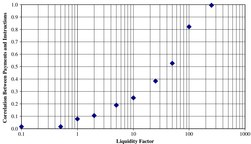
Fig. 4. Correlation coefficient between total payments sent and total instructions received in 2000 time intervals of size 10 for a range of liquidity factors. As liquidity decreases payments fail to track instructions as payment processing becomes governed by the coupling among banks.
