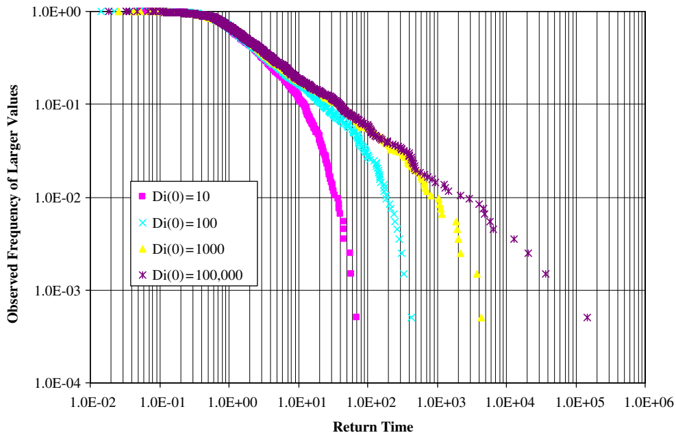
Fig. A.2. Frequency distributions of 1000 observations of return time \tau_r for four values of the deposit size D_i(0) . Including a finite deposit size introduces a roll-off in the return time distribution in the vicinity of D_i(0) .
