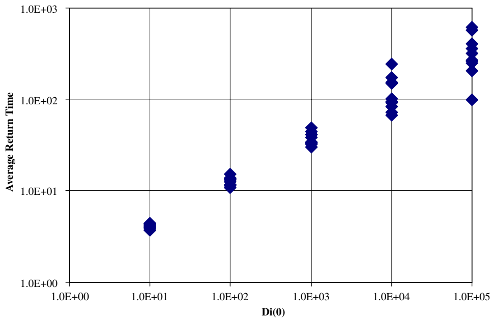
Fig. A.3. Averages of 1000 observations of return time \tau_r using various values of the deposit size D_i(0) . Ten averages from independent simulations are shown for each value of D_i(0) . The return time appears to scale with D_i^{\frac{1}{2}}(0) .
