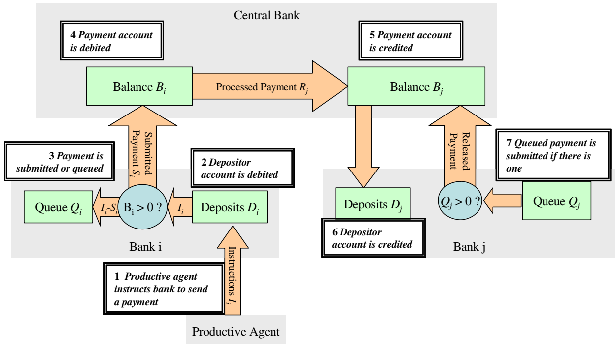
Fig. 1. Payment system components and state variables considered in the model, and their response to a payment instruction event.
