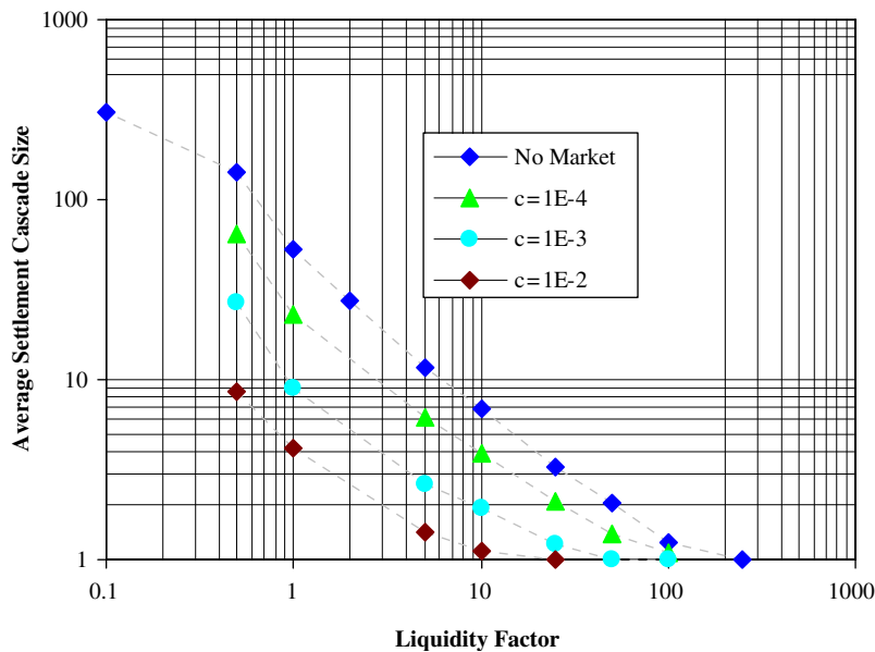
Fig. 10. Average cascade length as a function of liquidity factor for three values of market conductance. Results for the no-market case are included for comparison. The market model was not evaluated for liquidity factors of 2 and 0.1. Lines are a visual aid.
