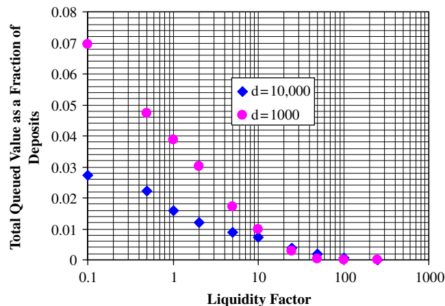
Fig. 21. Fraction of deposits in payment queues vs. liquidity factor for two deposit level values. Reducing deposits tends to increase the fraction of deposits queued. Although the absolute queue size is smaller with fewer deposits, the size relative to deposits is larger.
