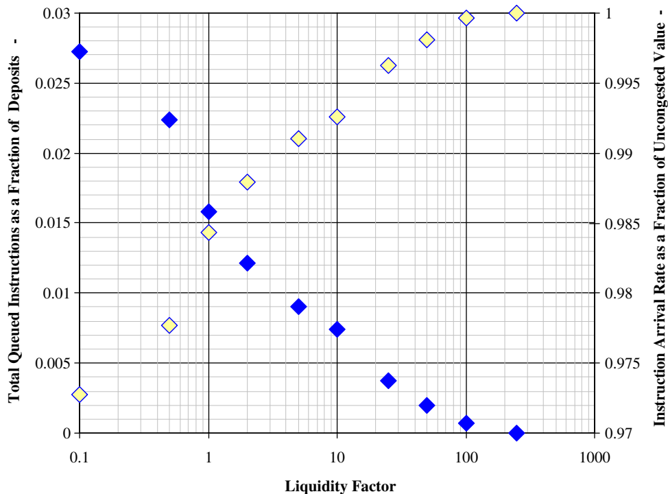
Fig. 7. Fraction of deposits in payment queues vs. liquidity factor (blue symbols, left scale) and instruction arrival rate as a fraction of the rate in an uncongested system (yellow symbols, right scale). The relative instruction arrival rate at a liquidity factor of 250 is plotted as 1 but is 1.00006 due to sampling variability.
