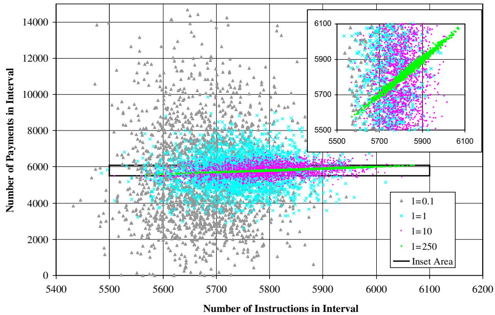
Fig. 3. Total number of instructions received and total number of payments settled in 2000 time intervals of size 10 for four values of the liquidity factor. The inset shows the center region using the same scale for instructions and payments. Payments track instructions at high liquidity; reducing liquidity causes periods of congestive delay and settlement cascades so that settlements are controlled by the dynamics of the coupled instruction queues and lose correlation with instructions. The average number of instructions also decreases at low liquidity as more deposits become trapped in payment queues: the center of the distribution of instructions shifts to the left as l decreases.
