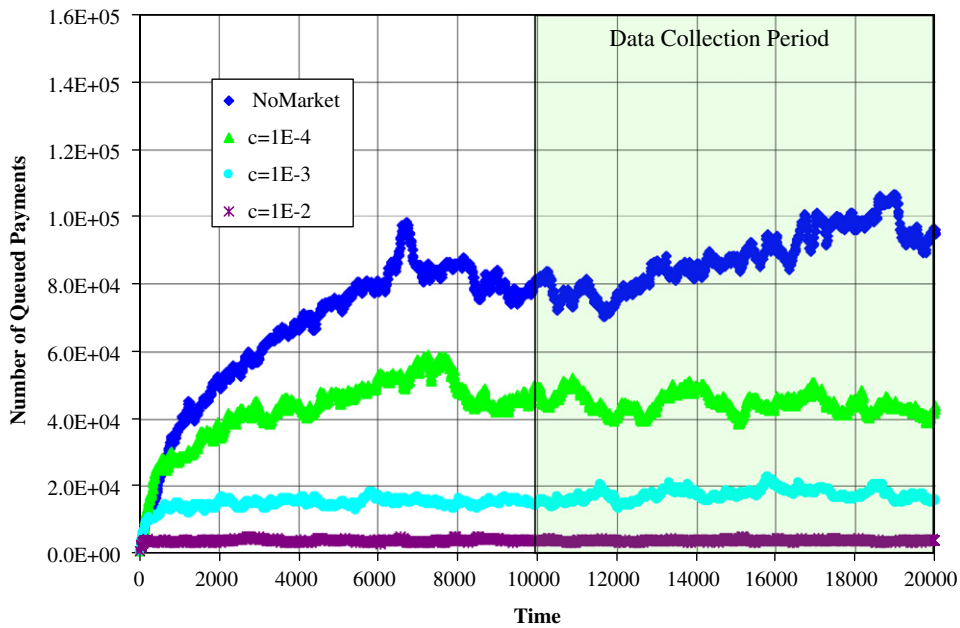
Fig. 9. Number of queued payments as a function of time for three values of market conductance c with a liquidity factor of 1. Results for the case with no market (dark blue symbols) are included for comparison. Higher conductance leads to smaller queues and more rapid stabilization.
