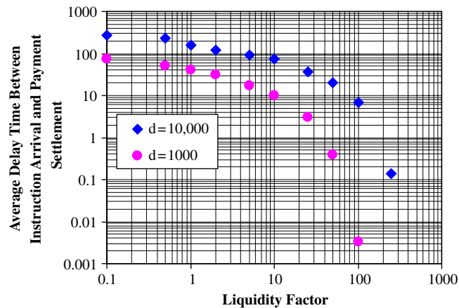
Fig. 22. Average delay time between instruction arrival and payment vs. liquidity factor for two deposit level values. At all liquidity levels delays are smaller with the lower deposit level.
