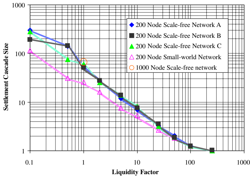
Fig. 15. Average size of settlement cascades observed in a time interval of length 20 000 for several values of the liquidity factor. Networks are distinguished by symbol. Lines indicate the analytical approximation for the expected value of cascade size from Eq. (16). The analytical approximation was only evaluated at the liquidity factor values used in the simulations: the lines are a visual aid. A range of liquidity factors was used in the three realizations of the 200-node network and the small world network; the 1000-node network was only simulated for l = 1 .
