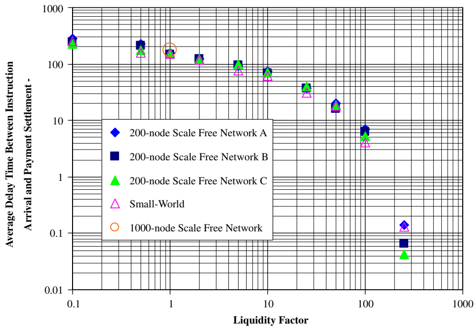
Fig. 18. Average delay time between instruction arrival and payment vs. liquidity factor for the alternative networks considered. Only small delay times, associated with large liquidity factors, appear to be sensitive to network structure.
