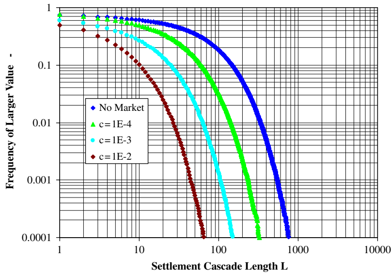
Fig. 11. Frequency distributions of observed cascade length with a liquidity factor of 1 for three values of market conductance. Results for the no-market case (dark blue symbols) are included for comparison. Observations were collected in a time period of 20 000 for the no-market case and in a period of 10 000 for the simulations including the market. Increasing c significantly reduces the size of settlement cascades.
