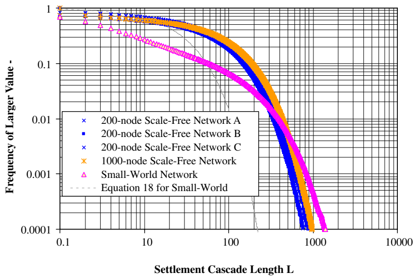
Fig. 16. Frequency distribution of observed cascade sizes for a liquidity factor of 1 for three realizations of the 200-node scale-free network (blue symbols), one realization of a 1000-node scale-free network (orange symbols), and one realization of a 200-node small-world network (pink symbols). The geometric distribution expected from the mean-field analysis for the small-world network is shown as a light grey line.
