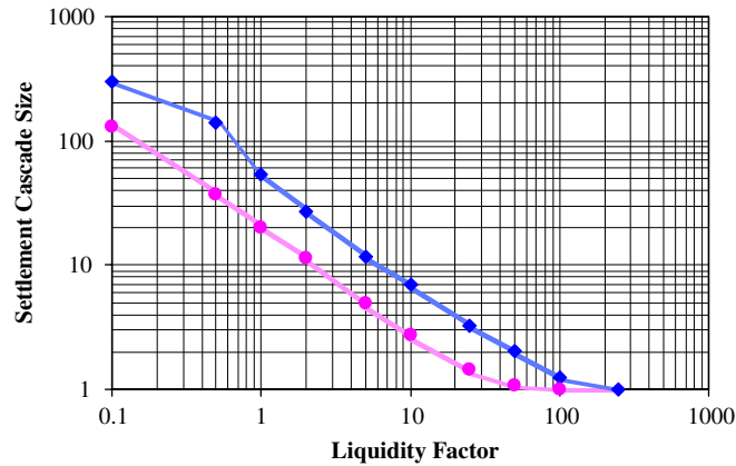
Fig. 19. Average size of settlement cascades observed in a time intervals of length 20 000 vs. liquidity factor for two deposit level values. Decreasing deposits decreases cascade size.
