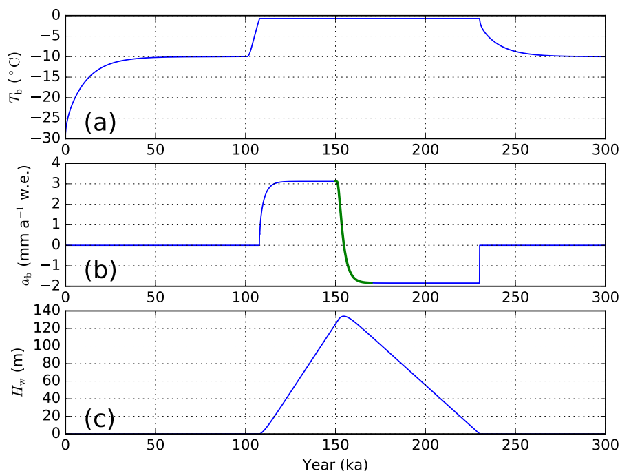
Figure 8. The result of (a) basal temperature ( T_b ), (b) basal melt rate ( a_b ), and (c) basal water thickness ( H_w ) for enthalpy benchmark experiment A. The green line from 150 to 170 ka in (b) indicates the analytical results (overlapped with model results).
