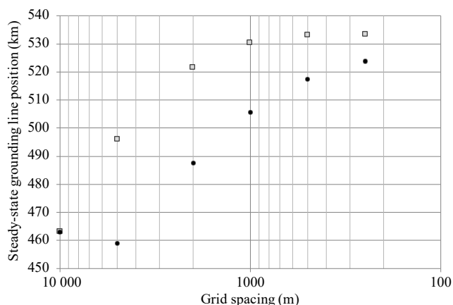
Figure 10. Grid resolution convergence for the MISMIP3d Stnd experiment with (gray squares) and without (black circles) grounding line parameterization.
