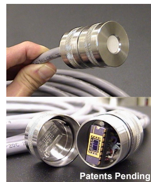
Weatherproof sensor package. The unique design and GORE-TEX ® membrane allows the enclosed chemiresistors to "sniff" chemicals in air, soil, and water environments.
