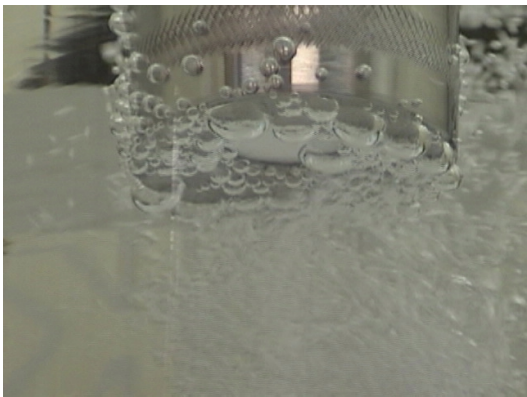
Bubbles accumulating on Gore-Tex ® membrane during underwater sparging. Bubbles dissolve as the gas partitions through membrane.
