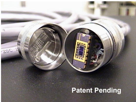
Sensor package taken apart, exposing chemiresistor sensor inside
